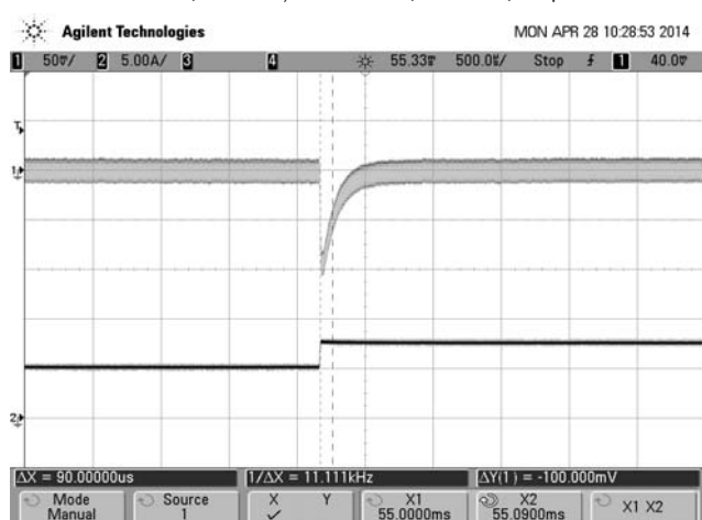
Step Load Transient Response (Vin=48V, Vout=nom., Cload=220uF, Iout=50% to 75% of full load, Ta=25° C) Trace 1=Vout, 50mV/div., 500uS/div.
