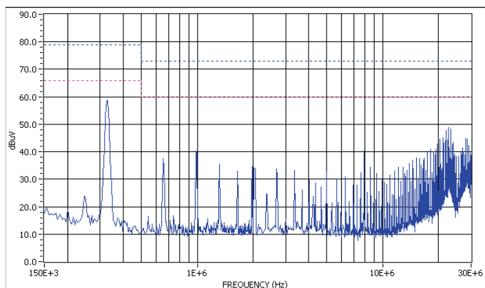
Graph 2. Conducted emissions performance, Negative Line, CISPR 22, Class A, full load
