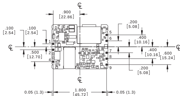
UEI50 Open Frame 50-60W
