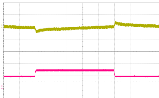
Fig. 12: Output voltage response to load current step-change (5 A – 7.5 A – 5 A) at V_{in} = 48\text{ V} . Top trace: output voltage (500 mV/div.). Bottom trace: load current (5 A/div.). Current slew rate: 1 A/ \mu\text{s} . C_o = 1\text{ }\mu\text{F} ceramic + 4,700 \mu\text{F} + 10 \mu\text{F} tantalum. Time scale: 200 \mu\text{s} /div.
