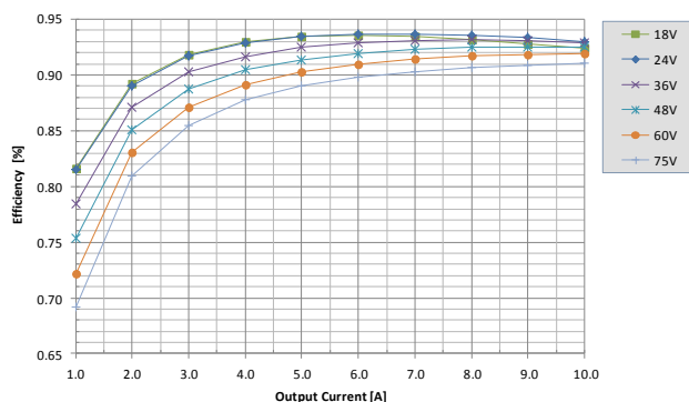
Fig. 7: Efficiency vs. load current and input voltage for UIE48T10120 converter w/o baseplate mounted vertically with air flowing from pin 3 to pin 1 at a rate of 300 LFM (1.5 m/s) and T_a = 25^\circ\text{C} .
