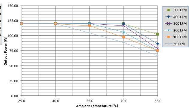
Fig. 2: Power derating vs. ambient air temperature and airflow rates for UIE48T10120 converter w/o baseplate mounted vertically with air flowing from pin 3 to pin 1, MOSFET temperature \leq 125^{\circ}\text{C} , V_{in}=48\text{V} .
