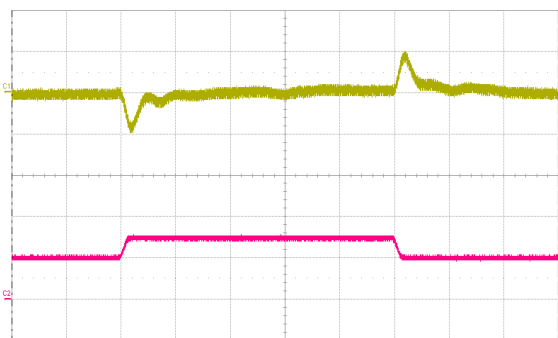
Fig. 11: Output voltage response to load current step-change (5 A – 7.5 A – 5 A) at V_{in} = 48\text{ V} . Top trace: output voltage (500 mV/div.). Bottom trace: load current (5 A/div.). Current slew rate: 0.1 A/ \mu\text{s} . C_o = 1\text{ }\mu\text{F} ceramic + 100 \mu\text{F} + 10 \mu\text{F} tantalum. Time scale: 200 \mu\text{s} /div.
