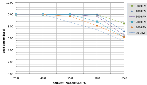
Fig. 1: Available load current vs. ambient air temperature and airflow rates for UIE48T10120 converter w/o baseplate mounted vertically with air flowing from pin 3 to pin 1, MOSFET temperature \leq 125^{\circ}\text{C} , V_{in}=48\text{V} .
