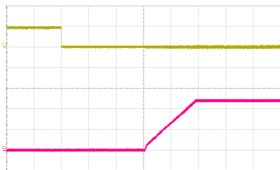
Fig. 9: Turn-on transient at full rated load current (resistive) with Cout 10 \mu\text{F} tantalum + 1 \mu\text{F} ceramic at V_{in} = 48\text{ V} , triggered via ON/OFF pin. Top trace: ON/OFF signal (5 V/div.). Bottom trace: output voltage (5 V/div.). Time scale: 20 ms/div.
