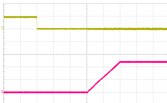
Fig. 10: Turn-on transient at full rated load current (resistive) plus 4,700 \mu\text{F} at V_{in} = 48\text{ V} , triggered via ON/OFF pin. Top trace: ON/OFF signal (5 V/div.). Bottom trace: output voltage (5 V/div.). Time scale: 20 ms/div.
