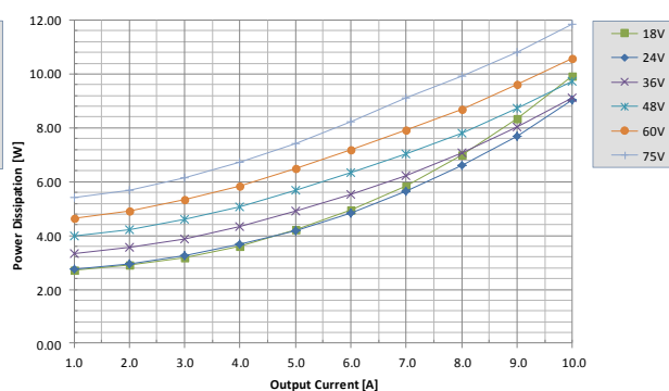
Fig. 8: Power dissipation vs. load current and input voltage for UIE48T10120 converter w/o baseplate mounted vertically with air flowing from pin 3 to pin 1 at a rate of 300 LFM (1.5 m/s) and T_a = 25^\circ\text{C} .
