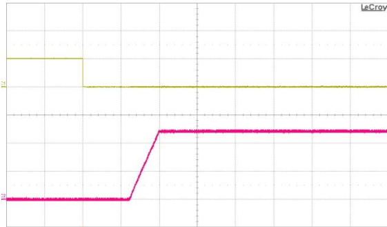
Fig. 9: Turn-on transient at full rated load current (resistive) with C_{out} 10 \mu F tantalum + 1 \mu F ceramic at V_{in} = 48 V, triggered via ON/OFF pin. Top trace: ON/OFF signal (5 V/div.). Bottom trace: output voltage (5 V/div.). Time scale: 50 ms/div.
