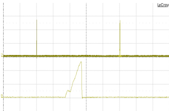
Fig. 17: Load current (top trace, 10 A/div., 100 ms/div.) into a 10 m \Omega short circuit during restart, at V_{in} = 48 V. Bottom trace (10 A/div., 10 ms/div.) is an expansion of the on-time portion of the top trace.
