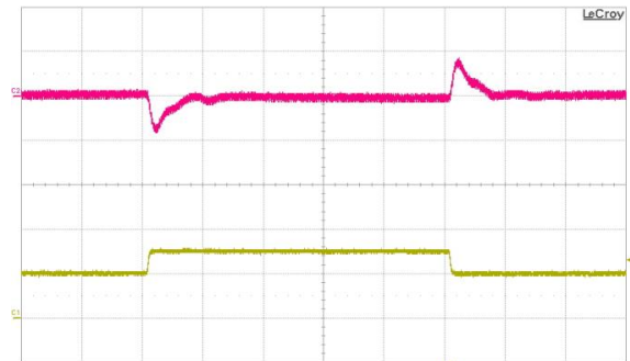
Fig. 12: Output voltage response to load current step change (10 A – 15 A – 10 A) at V_{in} = 48 V. Top trace: output voltage (500 mV/div.). Bottom trace: load current (10 A/div.). Current slew rate: 1 A/ \mu s. C_o = 1 \mu F ceramic + 4700 \mu F + 10 \mu F tantalum. Time scale: 200 \mu s/div.
