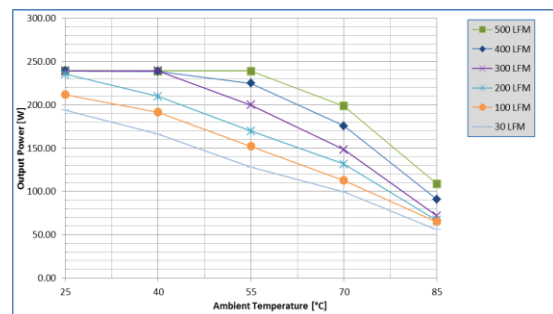
Fig. 2: Power derating vs. ambient air temperature and airflow rates for UIQ48T20120 converter w/o baseplate mounted vertically with air flowing from pin 3 to pin 1, MOSFET temperature \leq 125^\circ\text{C} , V_{in} = 48\text{V} .
