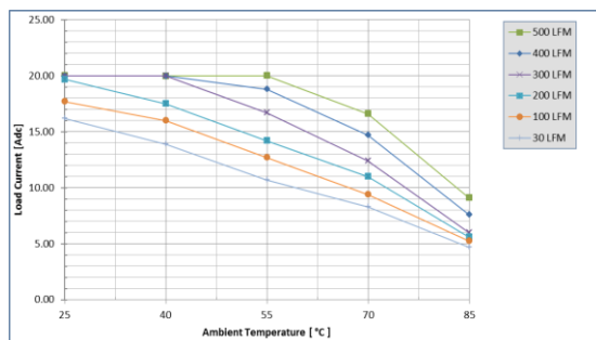
Fig. 1: Available load current vs. ambient air temperature and airflow rates for UIQ48T20120 converter w/o baseplate mounted vertically with air flowing from pin 3 to pin 1, MOSFET temperature \leq 125^\circ\text{C} , V_{in} = 48\text{V} .
