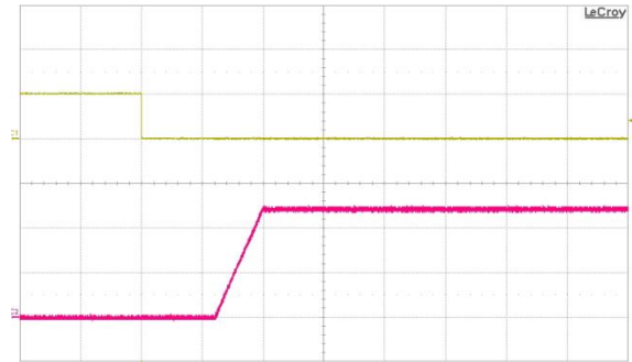
Fig. 10: Turn-on transient at full rated load current (resistive) plus 4700 \mu F at V_{in} = 48 V, triggered via ON/OFF pin. Top trace: ON/OFF signal (5 V/div.). Bottom trace: output voltage (5 V/div.). Time scale: 50 ms/div.
