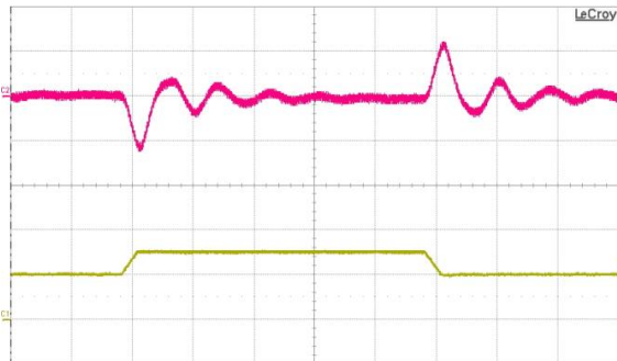
Fig. 11: Output voltage response to load current step change (10 A – 15 A – 10 A) at V_{in} = 48 V. Top trace: output voltage (500 mV/div.). Bottom trace: load current (10 A/div.). Current slew rate: 0.1 A/ \mu s. C_o = 1 \mu F ceramic + 10 \mu F tantalum. Time scale: 200 \mu s/div.
