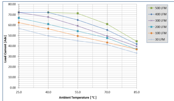
Fig. 3: Available load current vs. ambient air temperature and airflow rates for UIQ48T72033 converter w/o baseplate mounted vertically with air flowing from pin 3 to pin 1, MOSFET temperature \leq 125^{\circ}\text{C} , V_{in}=24\text{V}
