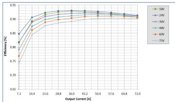
Fig. 7: Efficiency vs. load current and input voltage for UIQ48T72033 converter w/o baseplate mounted vertically with air flowing from pin 3 to pin 1 at a rate of 300 LFM (1.5 m/s) and T_a = 25^{\circ}\text{C} .
