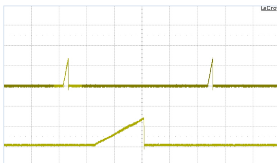
Fig. 17: Load current (top trace, 50 A/div., 100ms/div.) into a 10m \Omega short circuit during restart, at V_{in} = 48 V. Bottom trace (50 A/div., 10ms/div.) is an expansion of the on-time portion of the top trace
