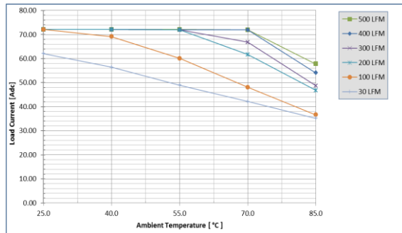
Fig. 5: Available load current vs. ambient air temperature and airflow rates for UIQ48T72033 converter with baseplate equipped with .45" finned heatsink mounted vertically with air flowing from pin 3 to pin 1, MOSFET temperature \leq 125^{\circ}\text{C} , V_{in}=48\text{V}
