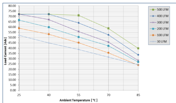
Fig. 1: Available load current vs. ambient air temperature and airflow rates for UIQ48T72033 converter w/o baseplate mounted vertically with air flowing from pin 3 to pin 1, MOSFET temperature \leq 125^\circ\text{C} , V_{in}=48\text{V}
