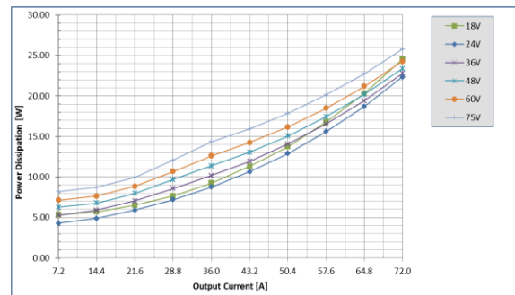
Fig. 8: Power dissipation vs. load current and input voltage for UIQ48T72033 converter w/o baseplate mounted vertically with air flowing from pin 3 to pin 1 at a rate of 300 LFM (1.5 m/s) and T_a = 25^{\circ}\text{C} .
