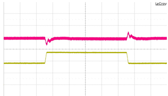
Fig. 12: Output voltage response to load current step change (36 A – 54 A – 36 A) at V_{in} = 48 V. Top trace: output voltage (500 mV/div.). Bottom trace: load current (20 A/div.). Current slew rate: 1 A/ \mu s. C_o = 1 \mu F ceramic + 10,000 \mu F tantalum. Time scale: 200 \mu s/div.
