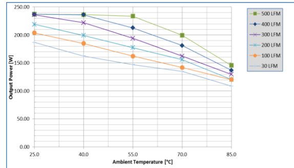
Fig. 4: Power derating vs. ambient air temperature and airflow rates for UIQ48T72033 converter w/o baseplate mounted vertically with air flowing from pin 3 to pin 1, MOSFET temperature \leq 125^{\circ}\text{C} , V_{in}=24\text{V}
