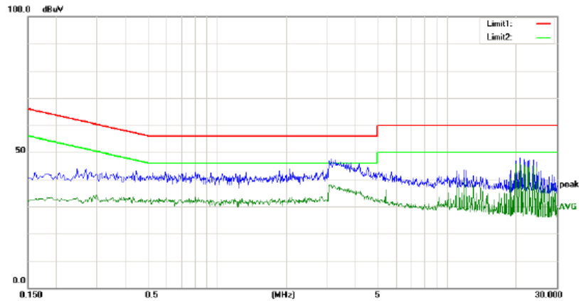
Fig. 20: Vin- Peak Detector EMI waveform
