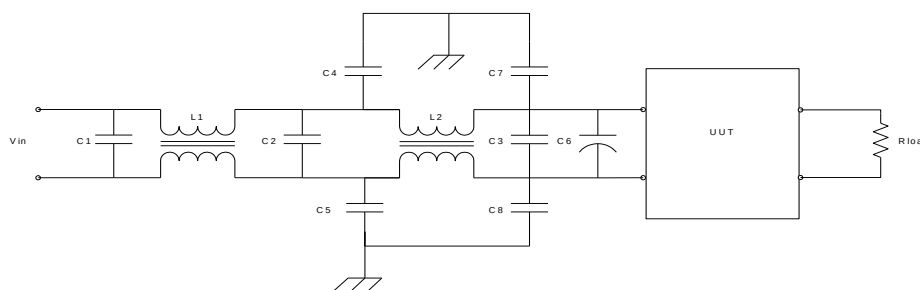
Fig. 18: Typical input EMI filter circuit to attenuate conducted emissions.
