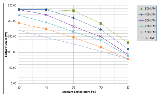
Fig. 2: Power derating vs. ambient air temperature and airflow rates for UIQ48T72033 converter w/o baseplate mounted vertically with air flowing from pin 3 to pin 1, MOSFET temperature \leq 125^\circ\text{C} , V_{in}=48\text{V}
