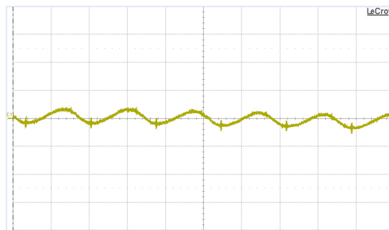
Fig. 16: Input reflected ripple current, i_s (20 mA/div.), measured through 10 \mu H at the source at full rated load current and V_{in} = 48 V. Refer to Fig. 14 for test setup. Time scale: 2 \mu s/div.
