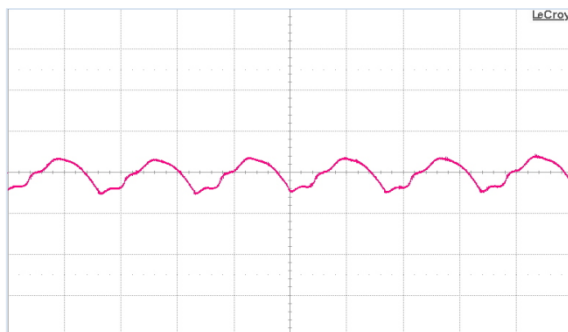
Fig. 13: Output voltage ripple (50 mV/div.) at full rated load current C_o = 10 \mu F tantalum + 1 \mu F ceramic and V_{in} = 48 V. Time scale: 2 \mu s/div.
