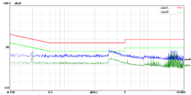
Fig. 19: Vin+ Peak Detector EMI waveform
