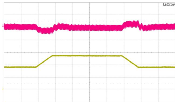
Fig. 11: Output voltage response to load current step change (36 A – 54 A – 36 A) at V_{in} = 48 V. Top trace: output voltage (200 mV/div.). Bottom trace: load current (20 A/div.). Current slew rate: 0.1 A/ \mu s. C_o = 1 \mu F ceramic + 10 \mu F tantalum. Time scale: 200 \mu s/div.
