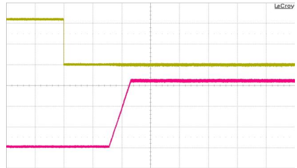
Fig. 10: Turn-on transient at full rated load current (resistive) plus 10,000 \mu F at V_{in} = 48 V, triggered via ON/OFF pin. Top trace: ON/OFF signal (2 V/div.). Bottom trace: output voltage (1 V/div.). Time scale: 50 ms/div.
