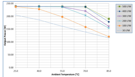
Fig. 6: Power derating vs. ambient air temperature and airflow rates for UIQ48T72033 converter with baseplate equipped with .45" finned heatsink mounted vertically with air flowing from pin 3 to pin 1, MOSFET temperature \leq 125^{\circ}\text{C} , V_{in}=48\text{V}
