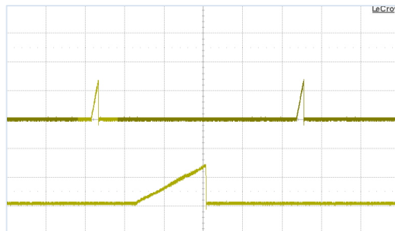
Fig. 17: Load current (top trace, 50 A/div., 100ms/div.) into a 10\text{m}\Omega short circuit during restart, at V_{in} = 48 \text{ V} . Bottom trace (50 A/div., 10ms/div.) is an expansion of the on-time portion of the top trace
