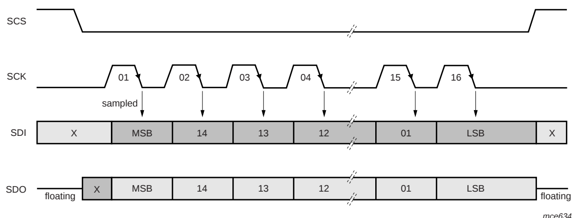
Fig 14. SPI timing protocol
