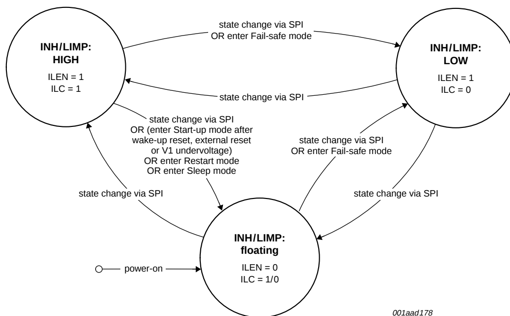
Fig 12. States of the INH/LIMP pin
