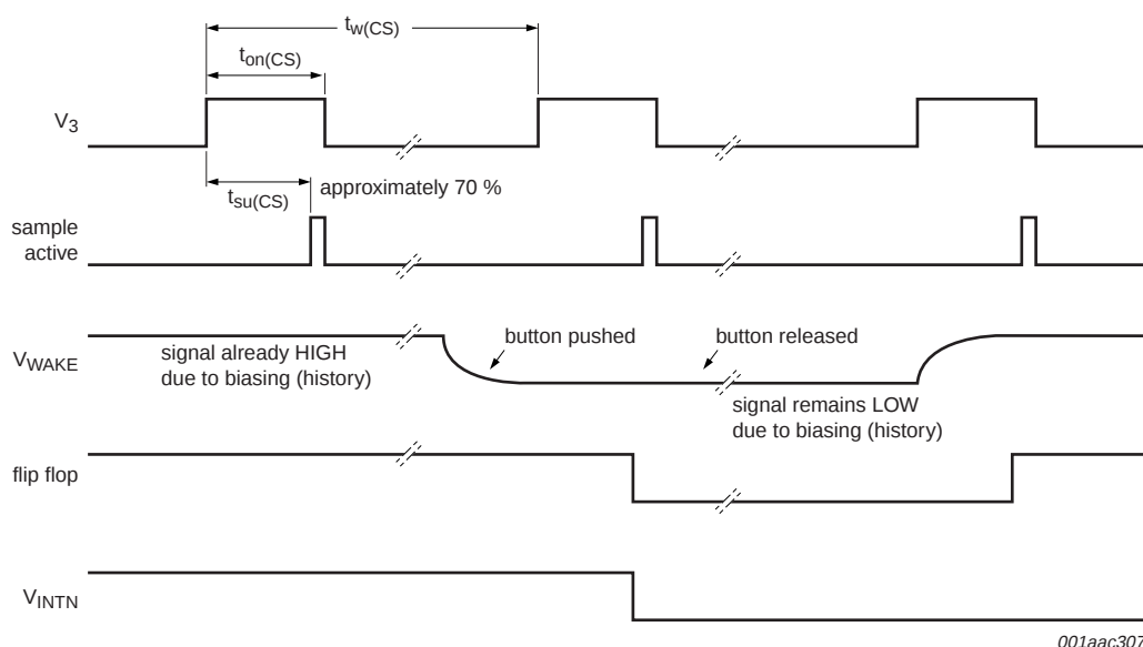
Fig 13. Pin WAKE, cyclic sampling via V3
