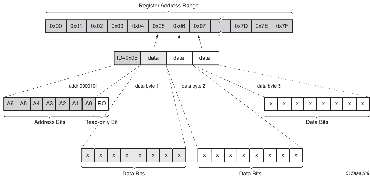
Fig 12. SPI data structure for a write operation (16-, 24- or 32-bit)
