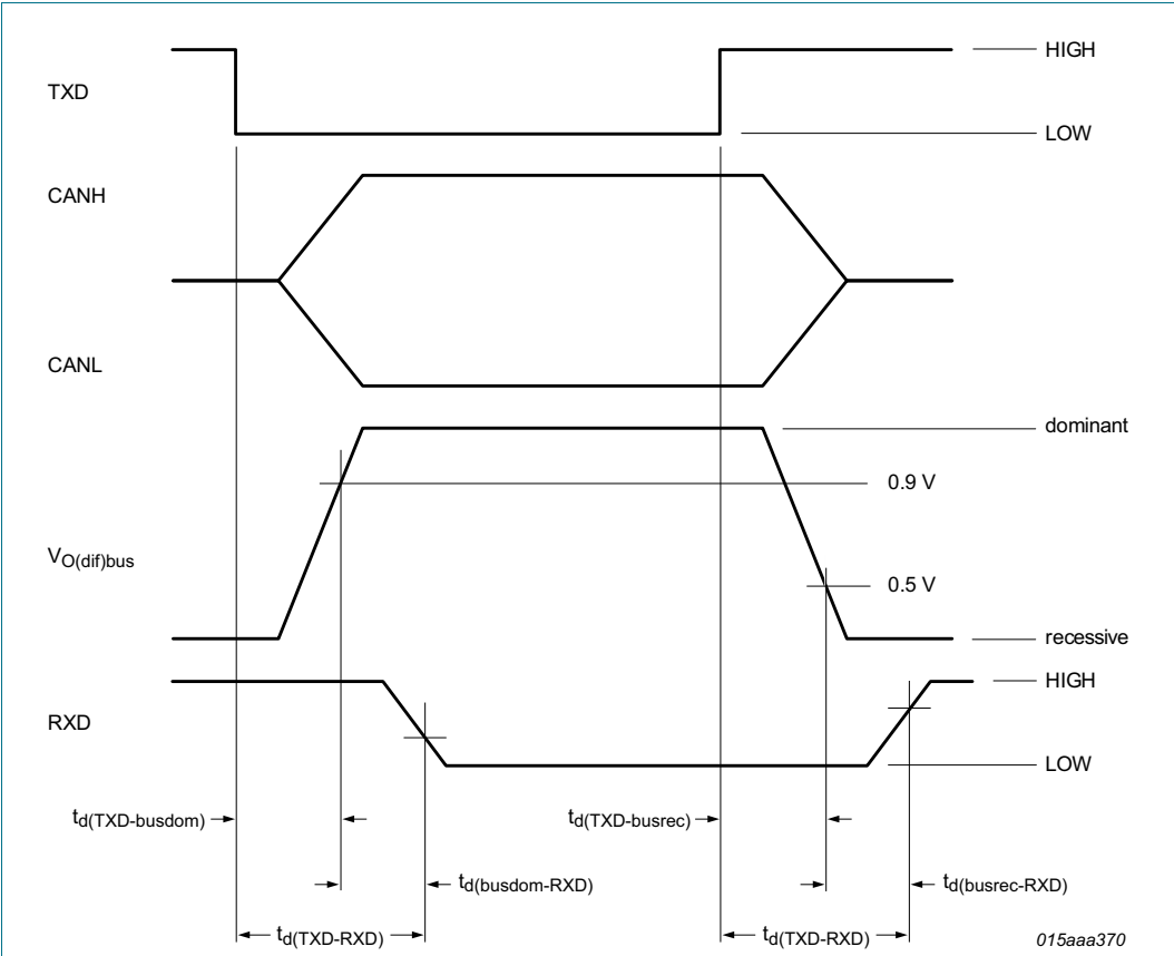
Fig 13. CAN transceiver timing diagram
