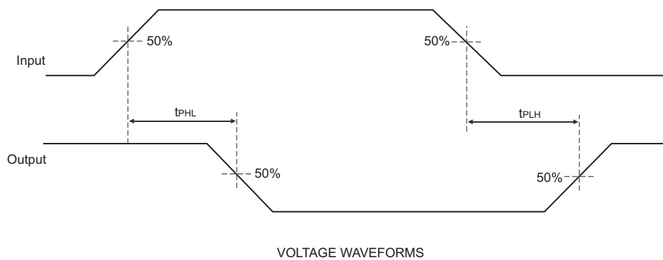
Figure 9. Propagation Delay-Time Waveforms
