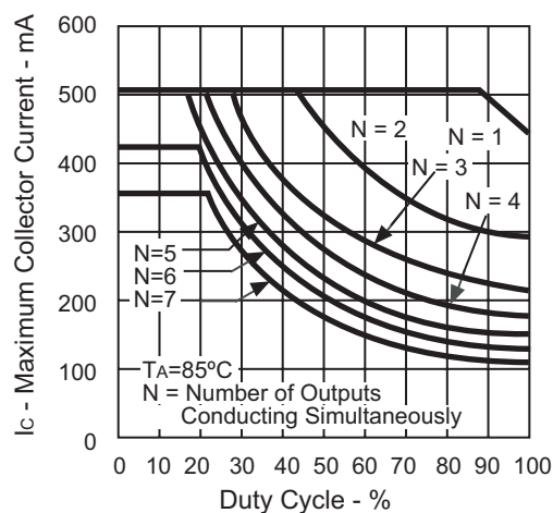
Figure 15. N PACKAGE MAXIMUM COLLECTOR CURRENT vs. DUTY CYCLE
