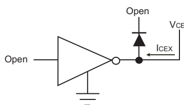
Figure 1. I_{CEX} Test Circuit
