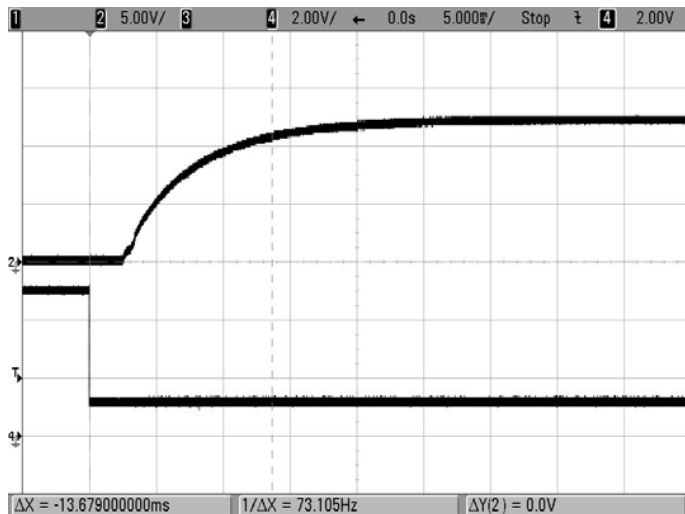
Enable Start-up (Vin=48V, Iout=5A, Cload=1000μF Ta=+25°C) Trace 2=Output, Trace 4= Enable.
