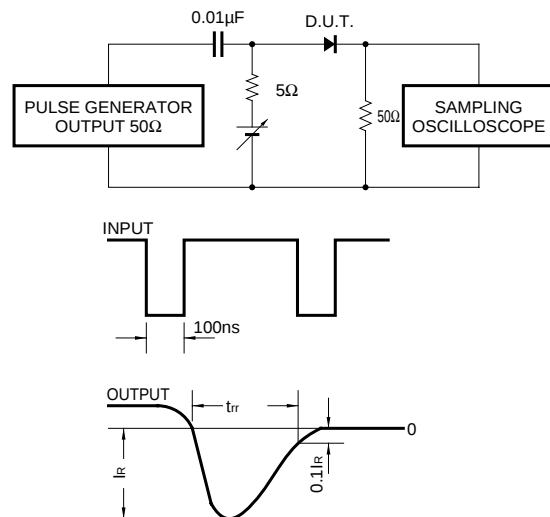
Fig.14 Reverse recovery time ( t_{rr} ) measurement circuit
