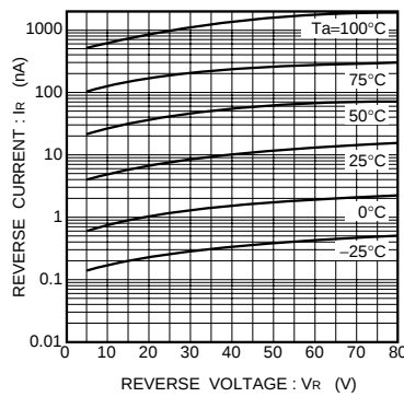
Fig.11 Reverse characteristics
