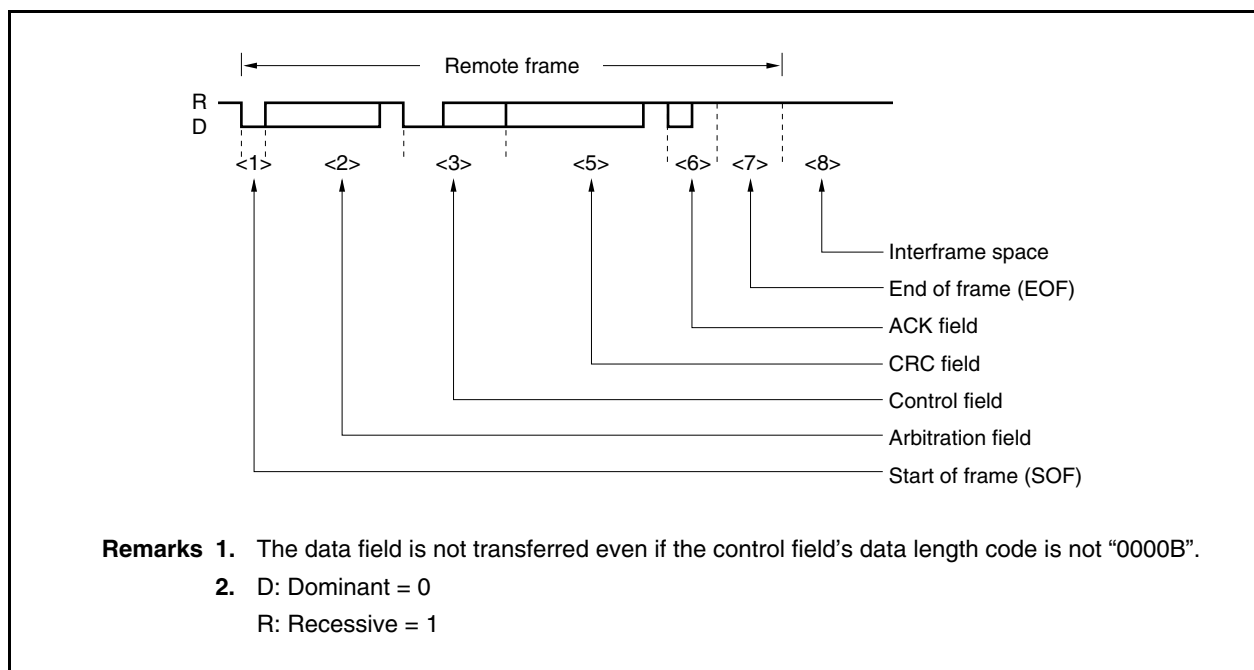
Figure 19-4. Remote Frame
