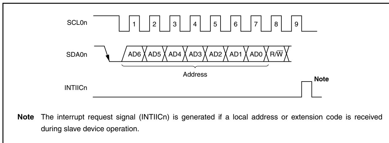
Figure 18-9. Address
