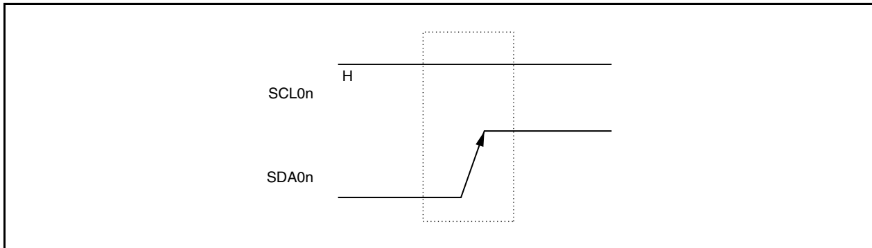
Figure 18-12. Stop Condition
