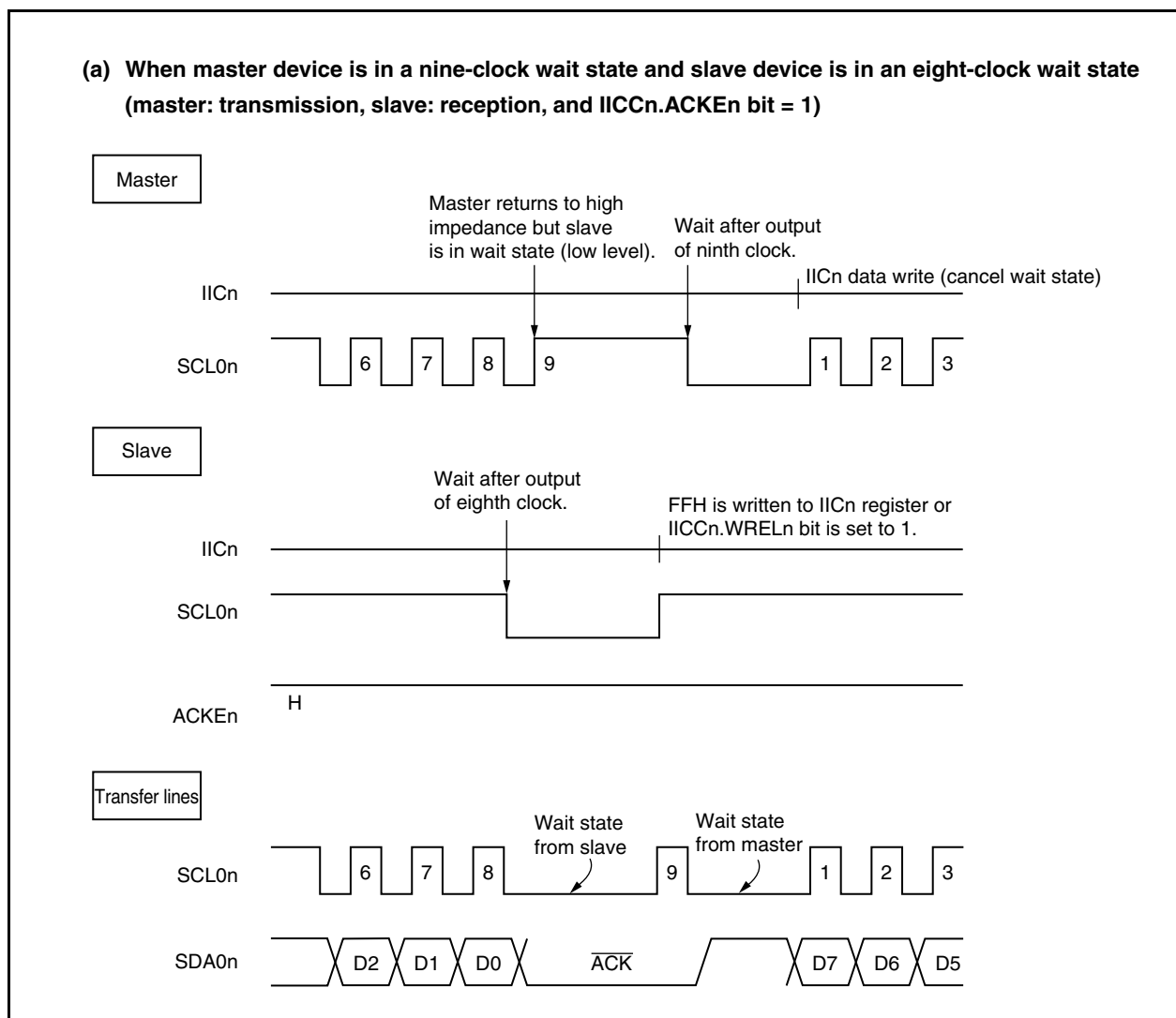
Figure 18-13. Wait State (1/2)
