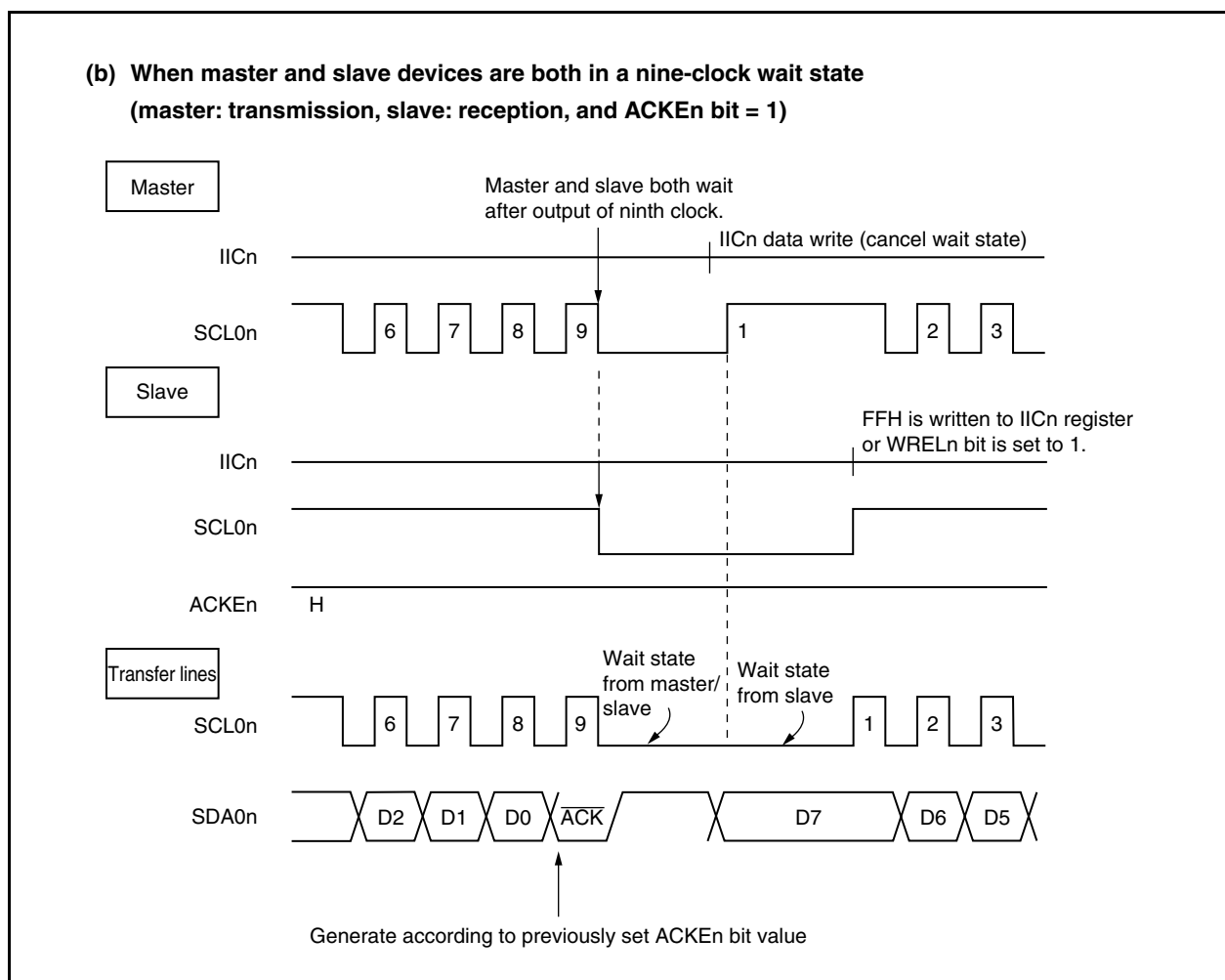
Figure 18-13. Wait State (2/2)
