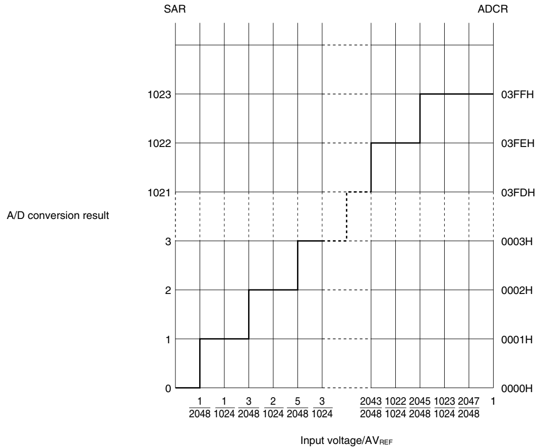
Figure 11-17. Relationship between Analog Input Voltage and A/D Conversion Result
