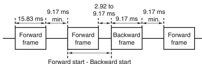
Figure 14-29. Timing among frames
