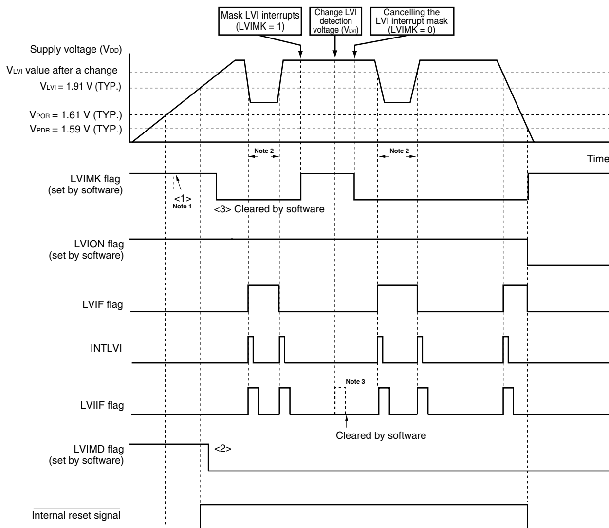
Figure 22-7. Timing of Low-Voltage Detector Interrupt Signal Generation (LVISTART = 1)
