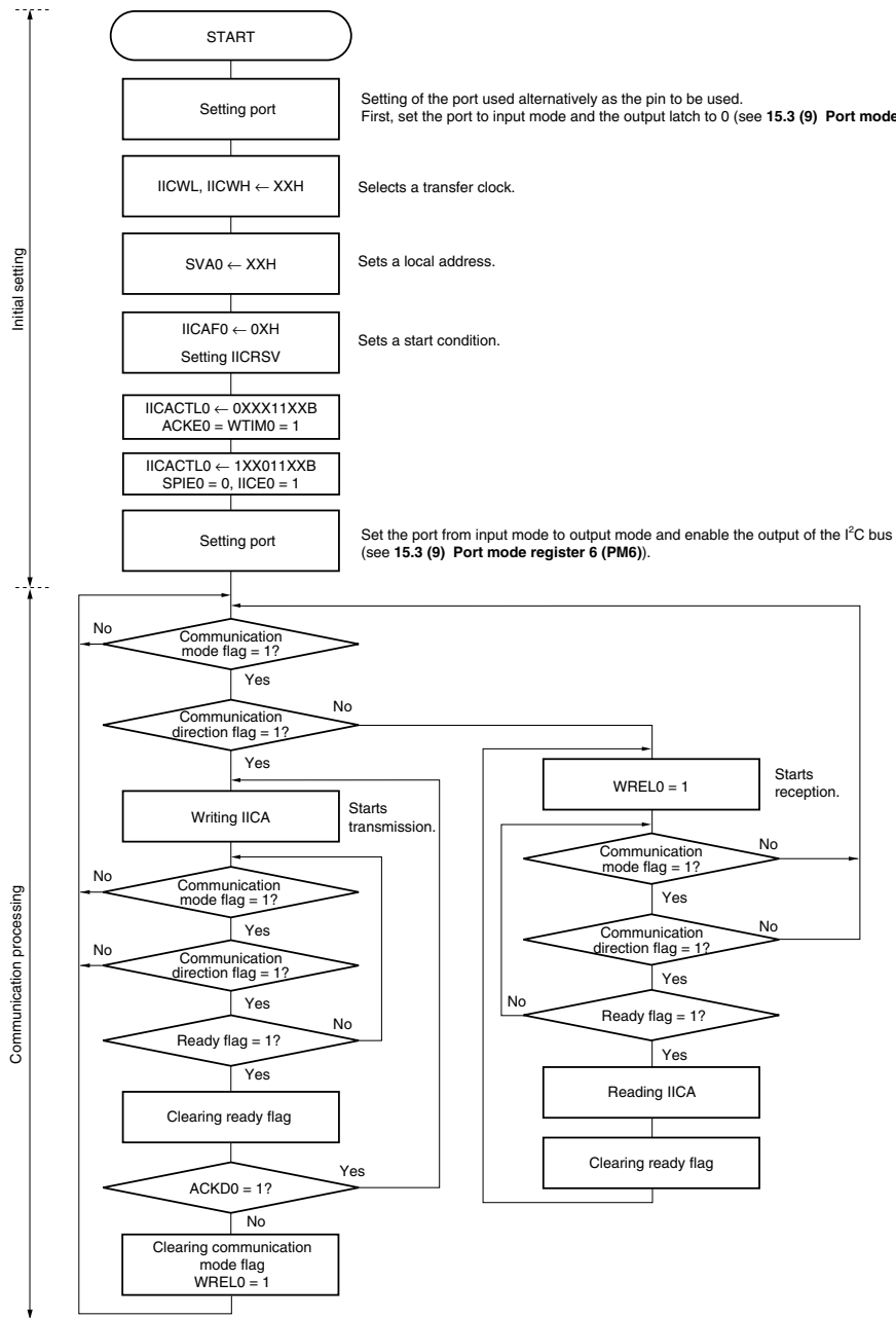
Figure 15-32. Slave Operation Flowchart (1)
