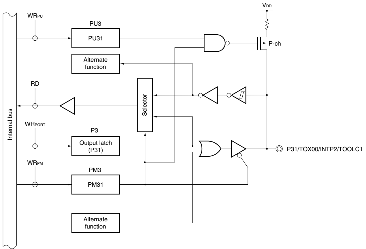
Figure 4-13. Block Diagram of P31
