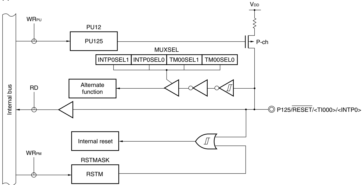
Figure 4-24. Block Diagram of P125
