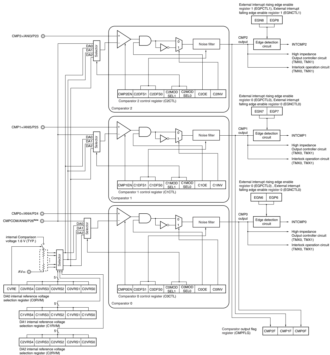
Figure 13-1. Block Diagram of Comparator/Programmable Gain Amplifier
