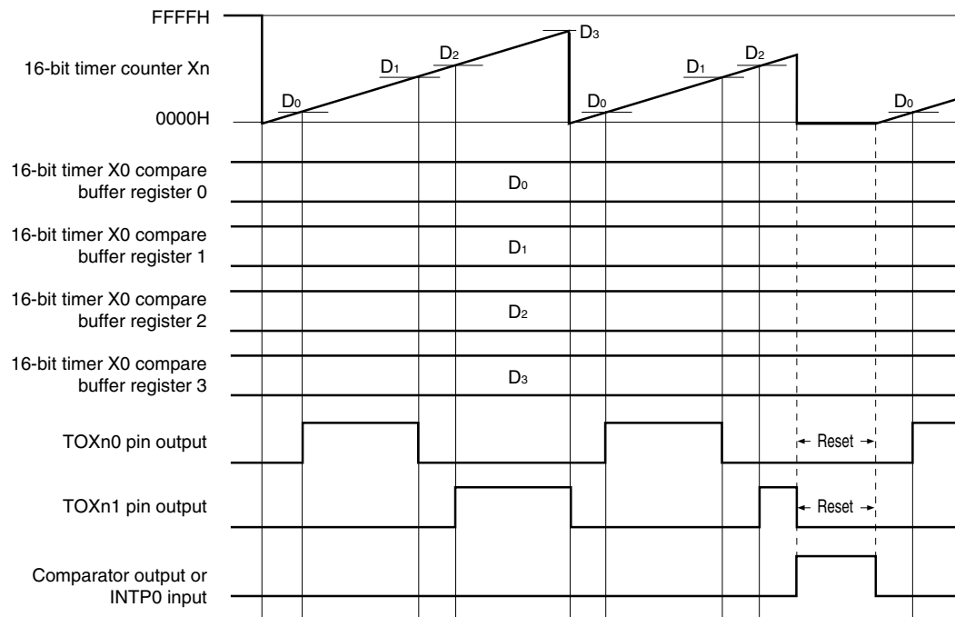
Figure 6-38. Timing of Interlocking mode 1 (timer reset mode)
