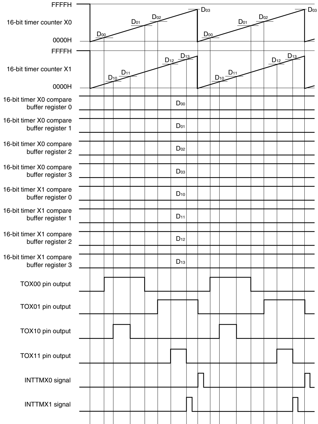
Figure 6-23. PWM Output Timing (TMX0 and TMX1 synchronous start/clear mode, PWM output: TOX00, TOX01, TOX10, and TOX11 pins)
