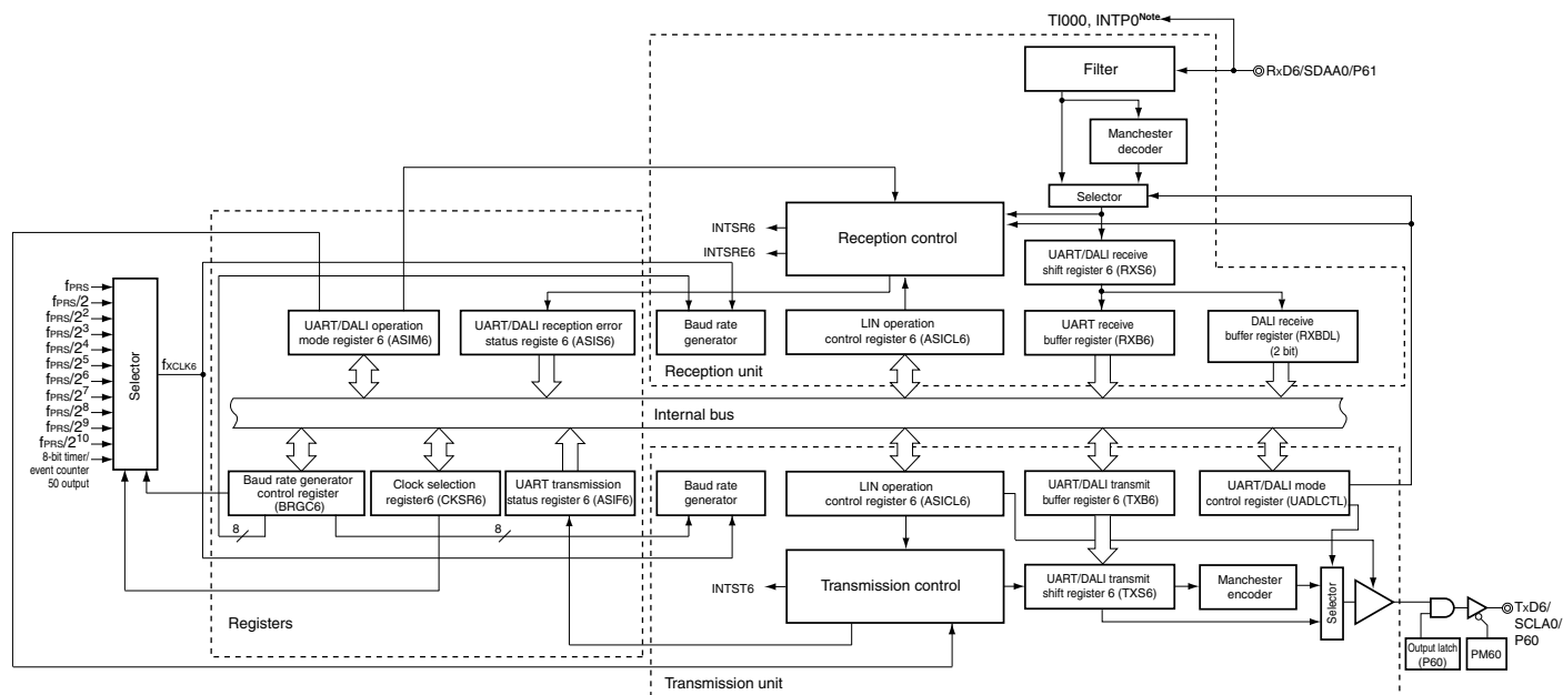
Figure 14-4. Block Diagram of Serial Interface UART6/DALI
