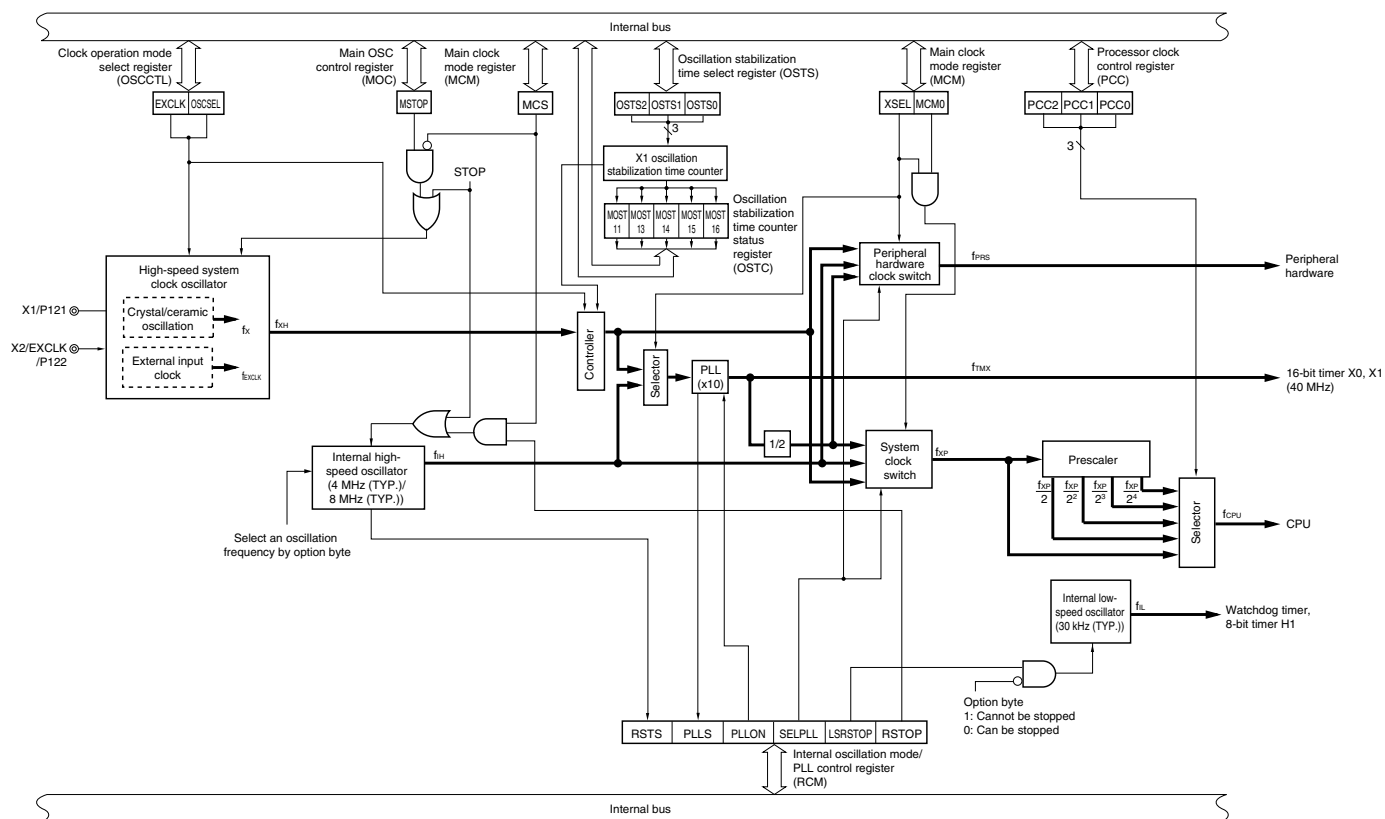
Figure 5-1. Block Diagram of Clock Generator
