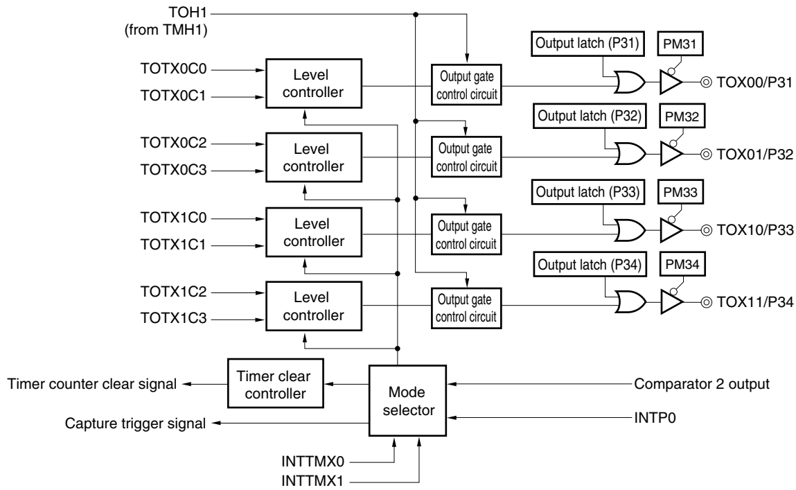
Figure 6-36. Block Diagram of 16-Bit Timers X0 and X1 Output Configuration
