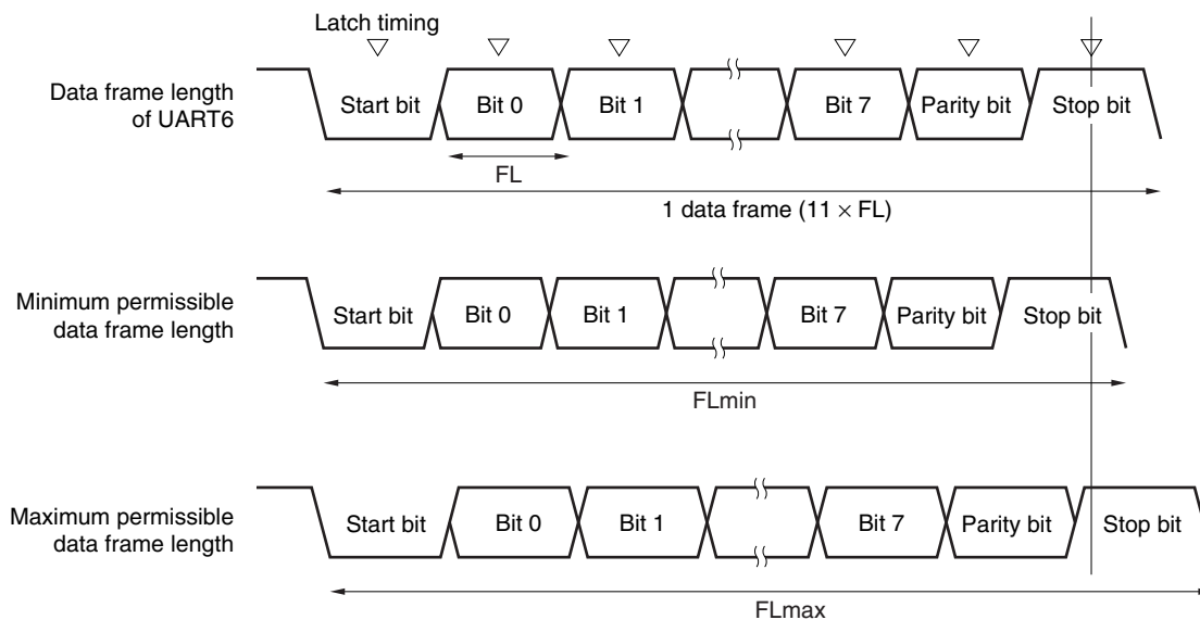
Figure 14-34. Permissible Baud Rate Range During Reception
