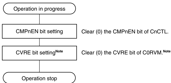
Figure 13-14. Example of Setting Procedure when Stopping Comparator Operation
