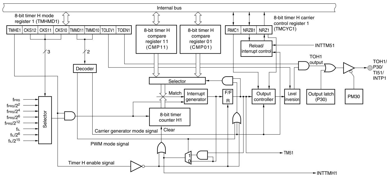
Figure 9-1. Block Diagram of 8-Bit Timer H1
