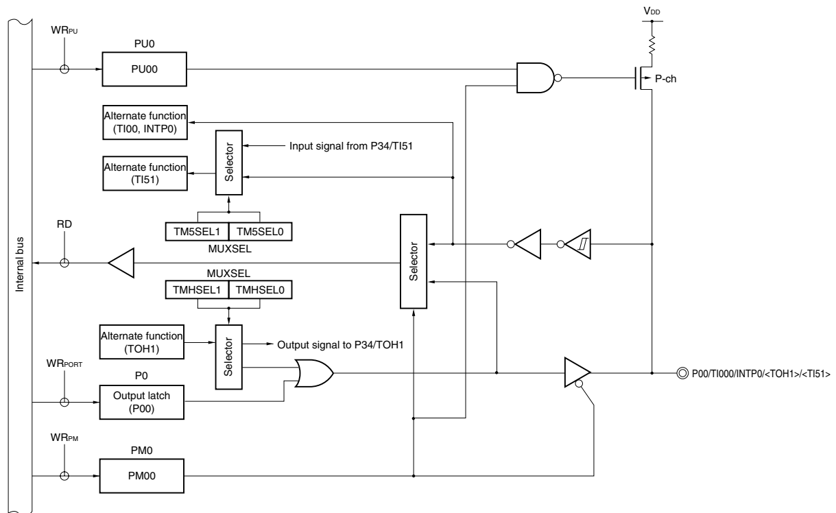
Figure 4-1. Block Diagram of P00 (1/2)
