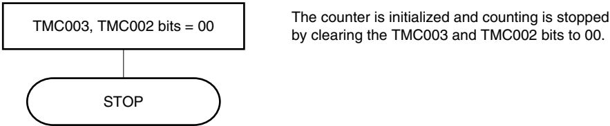
<2> Count operation stop flow
