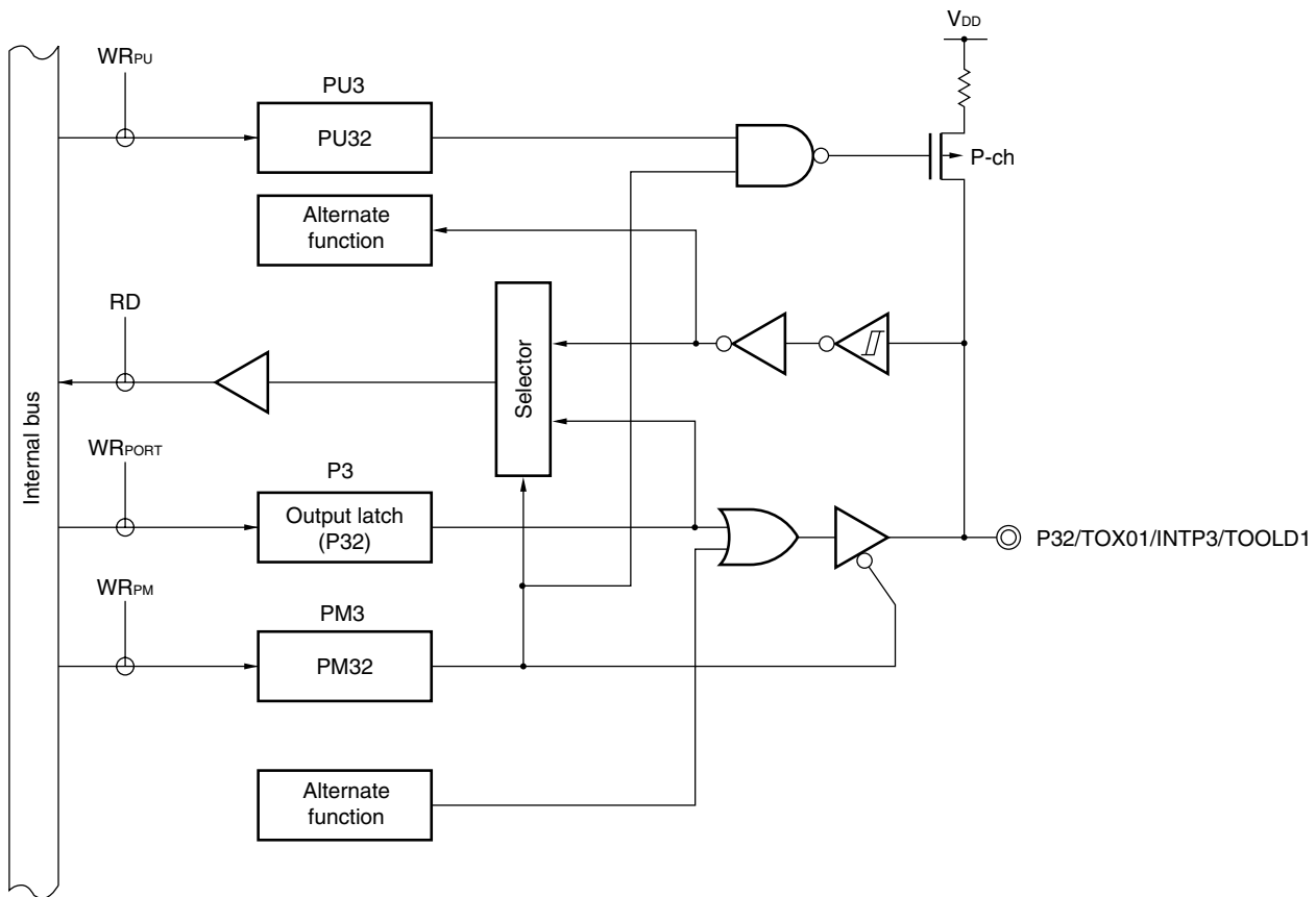
Figure 4-14. Block Diagram of P31
