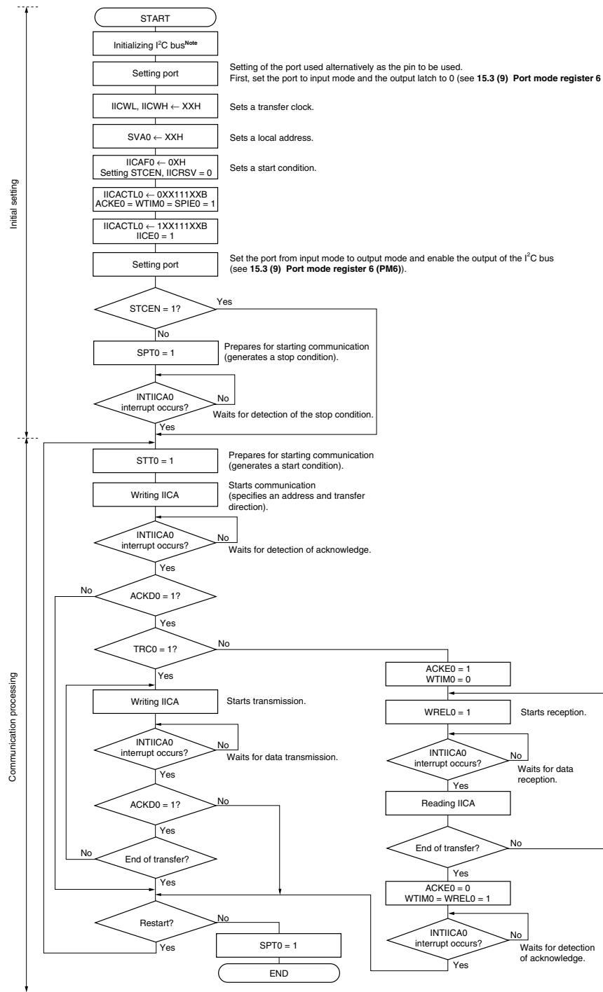
Figure 15-30. Master Operation in Single-Master System
