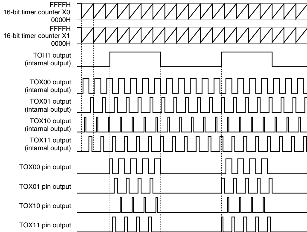
Figure 6-33. PWM Output Timing (TMX0 and TMX1 synchronous start/clear mode, PWM Output from TOX00, TOX01, TOX10, and TOX11 When TOH1 Output Is at High Level)
