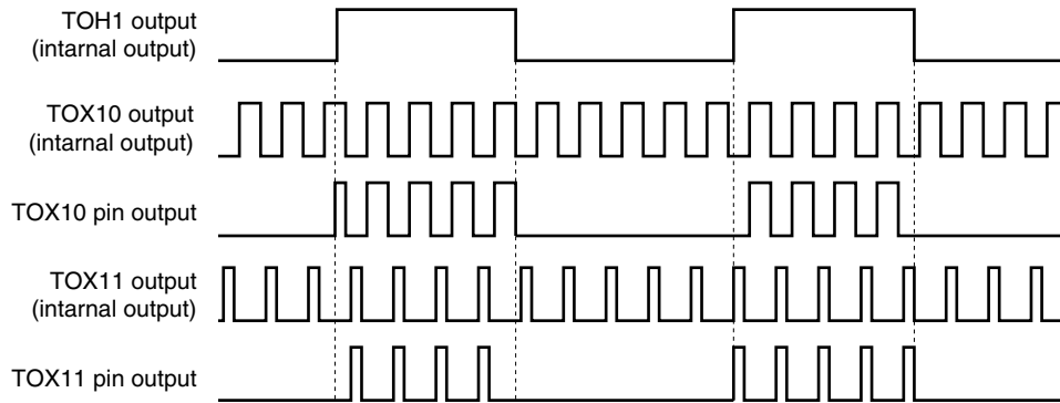
Figure 6-31. PWM Output Timing (TMX1-Only Operation (Dual Output), PWM Output from TOX10 and TOX11 When TOH1 Output Is at High Level)
