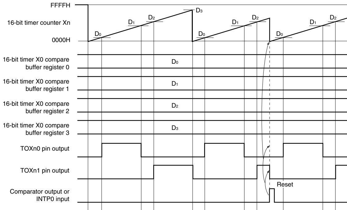
Figure 6-40. Timing of Interlocking mode 2 (timer restart mode)
