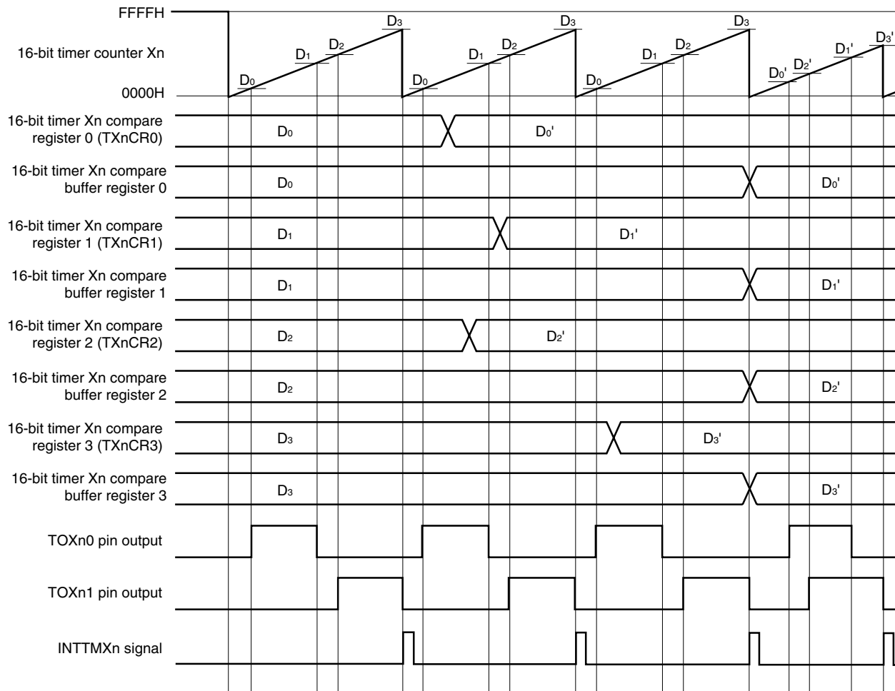
Figure 6-21. PWM Output Timing (TMXn-only Operation, PWM output: TOXn0 and TOXn1 pins)
