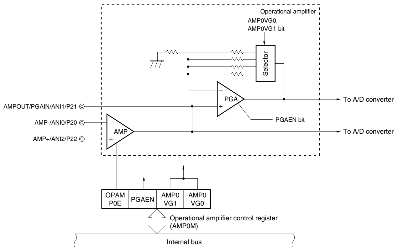
Figure 12-1. Block Diagram of Operational Amplifier
