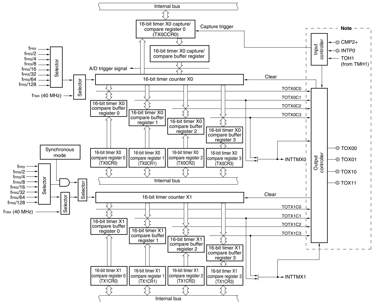
Figure 6-3. Block Diagram of 16-Bit Timers X0 and X1 (TMX0 and TMX1 Synchronous Start/clear Mode, TMX0 and TMX1 Synchronous Start Mode)
