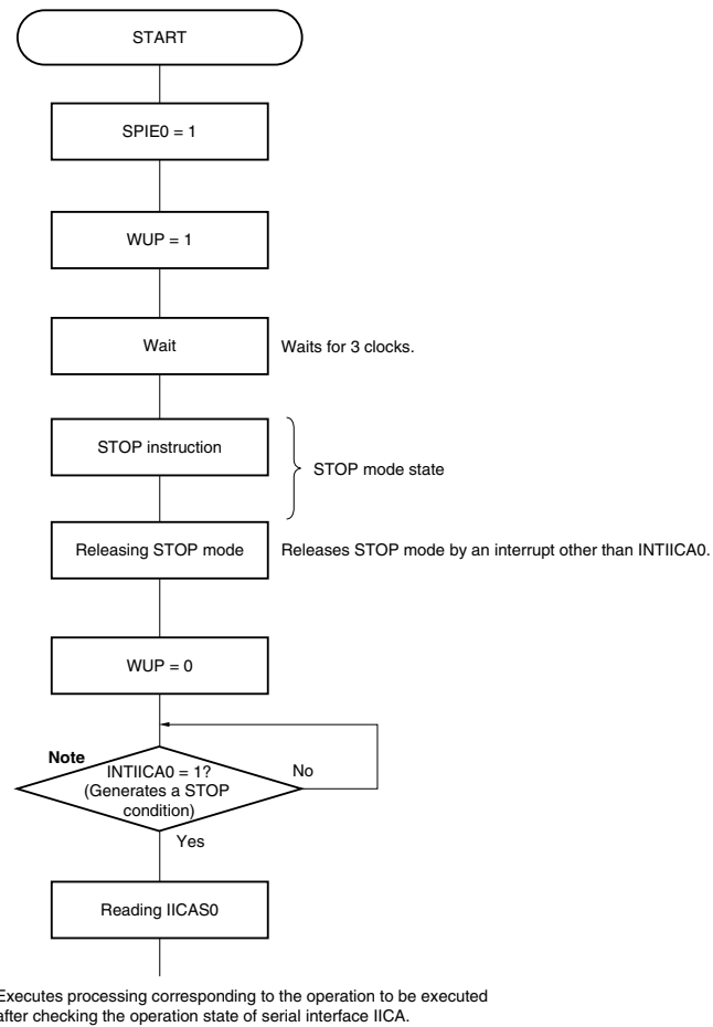
Figure 15-25. When Operating as Master Device after Releasing STOP Mode other than by INTIICA0
