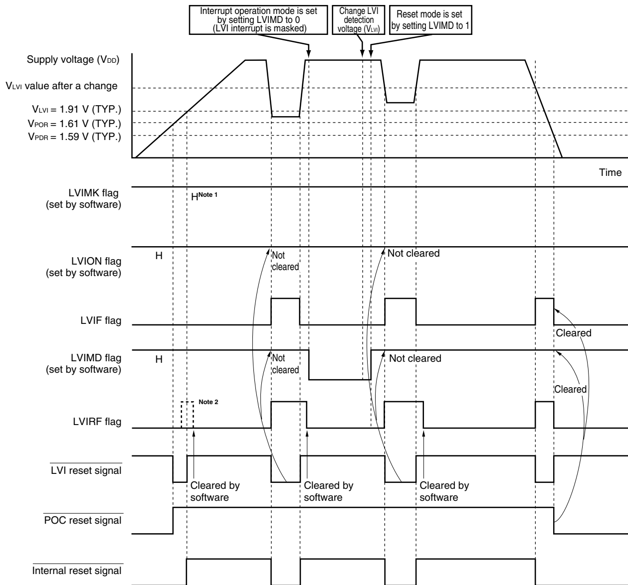
Figure 22-5. Timing of Low-Voltage Detector Internal Reset Signal Generation (LVISTART = 1)
