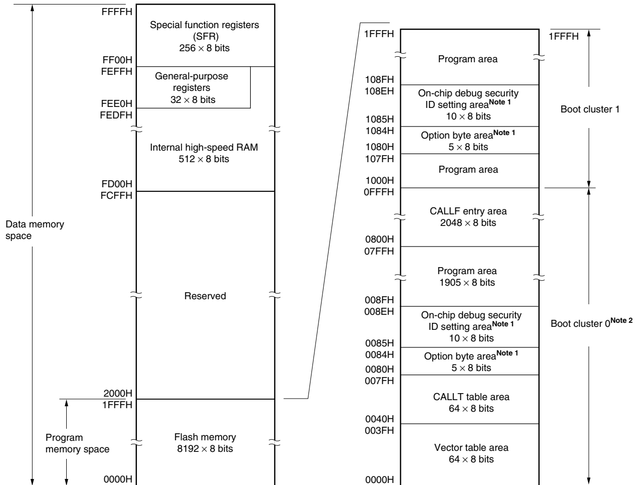
Figure 3-2. Memory Map (μPD78F0741, 78F0743, 78F0745, 78F0751, 78F0753, 78F0755)
