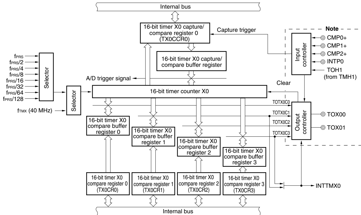
Figure 6-1. Block Diagram of 16-Bit Timer X0
