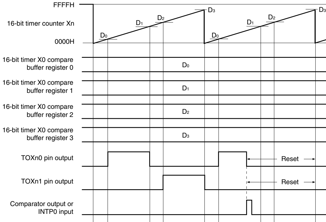
Figure 6-42. Timing of Interlocking mode 3 (timer output reset mode)
