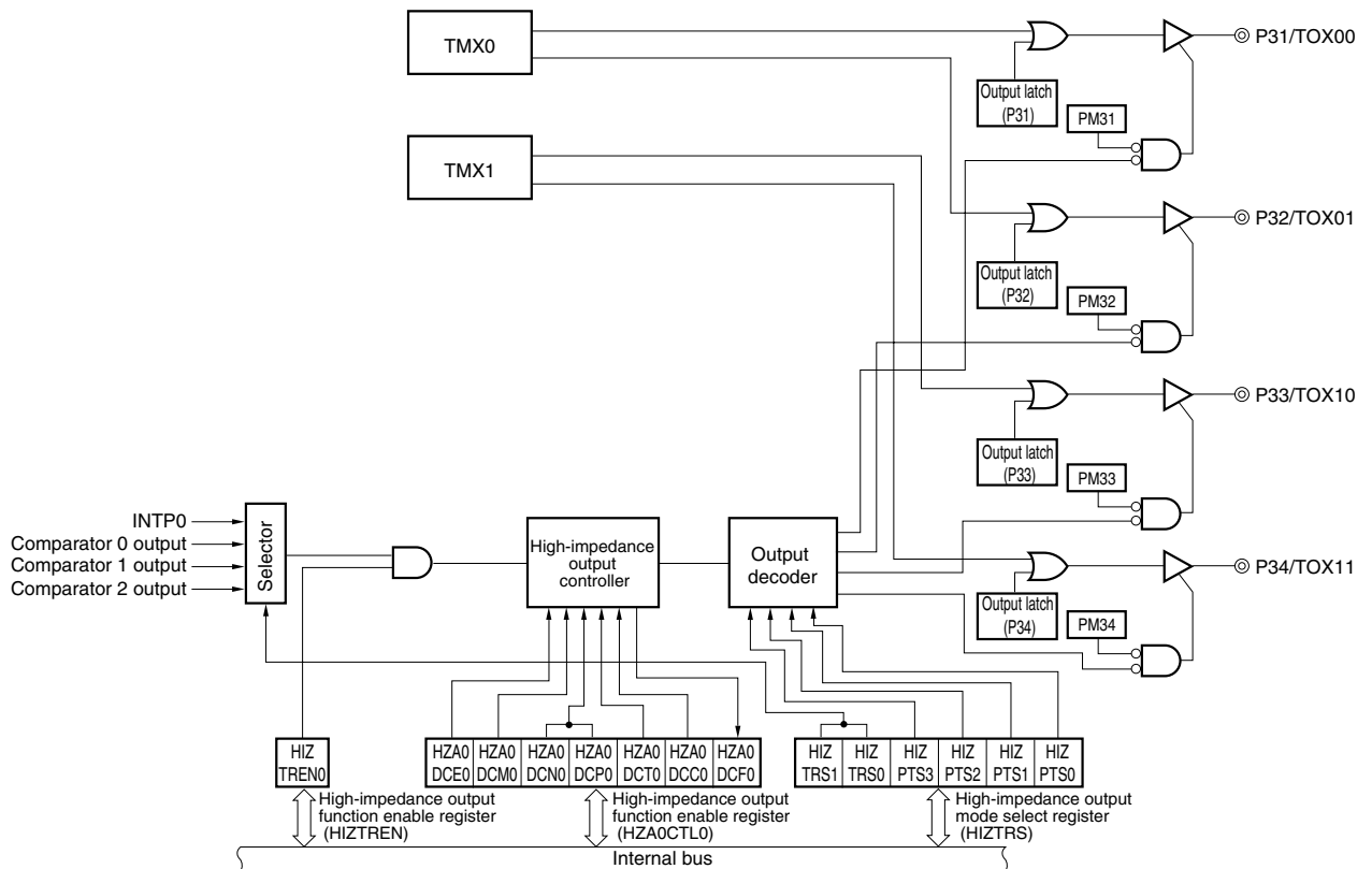
Figure 6-43. Block Diagram of High-Impedance Output Controller
