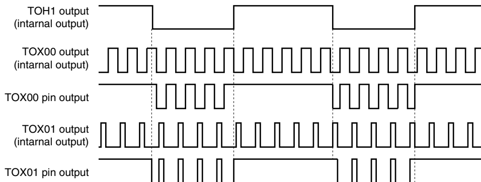
Figure 6-29. PWM Output Timing (TMX0-Only Operation (Dual Output), PWM Output from TOX00 and TOX01 When TOH1 Output Is at Low Level)
