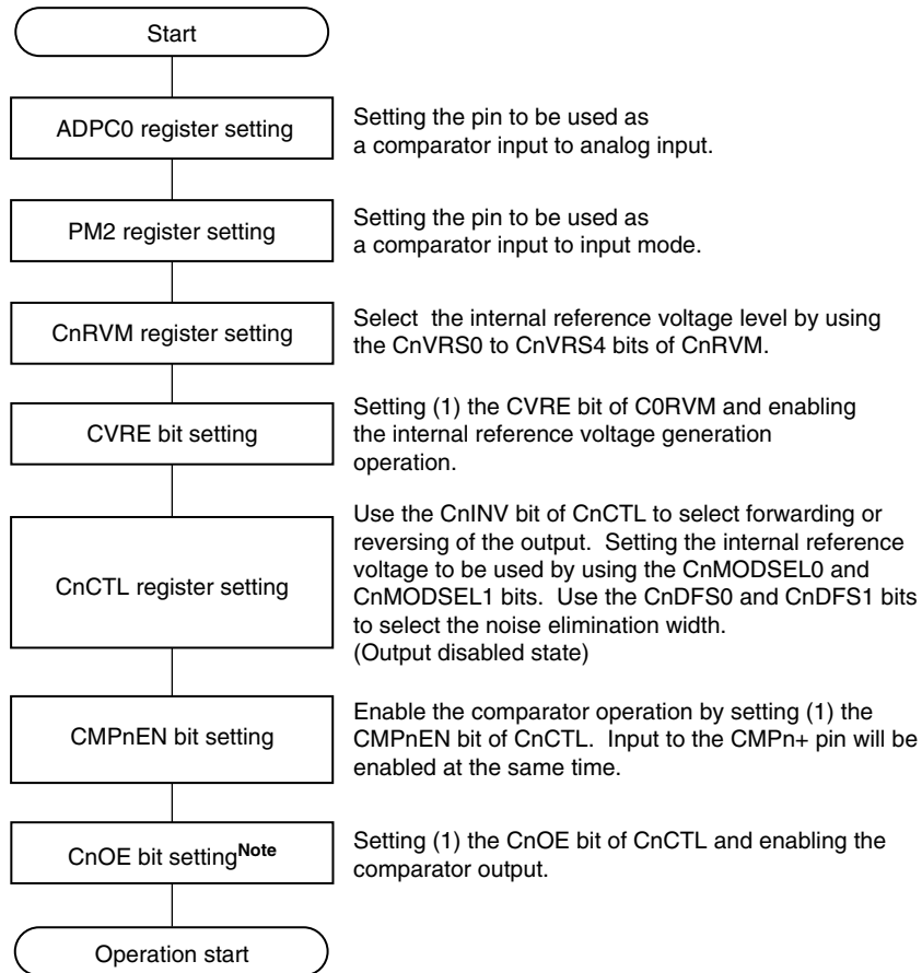
Figure 13-12. Example of Setting Procedure when Changing Internal Reference Voltage
