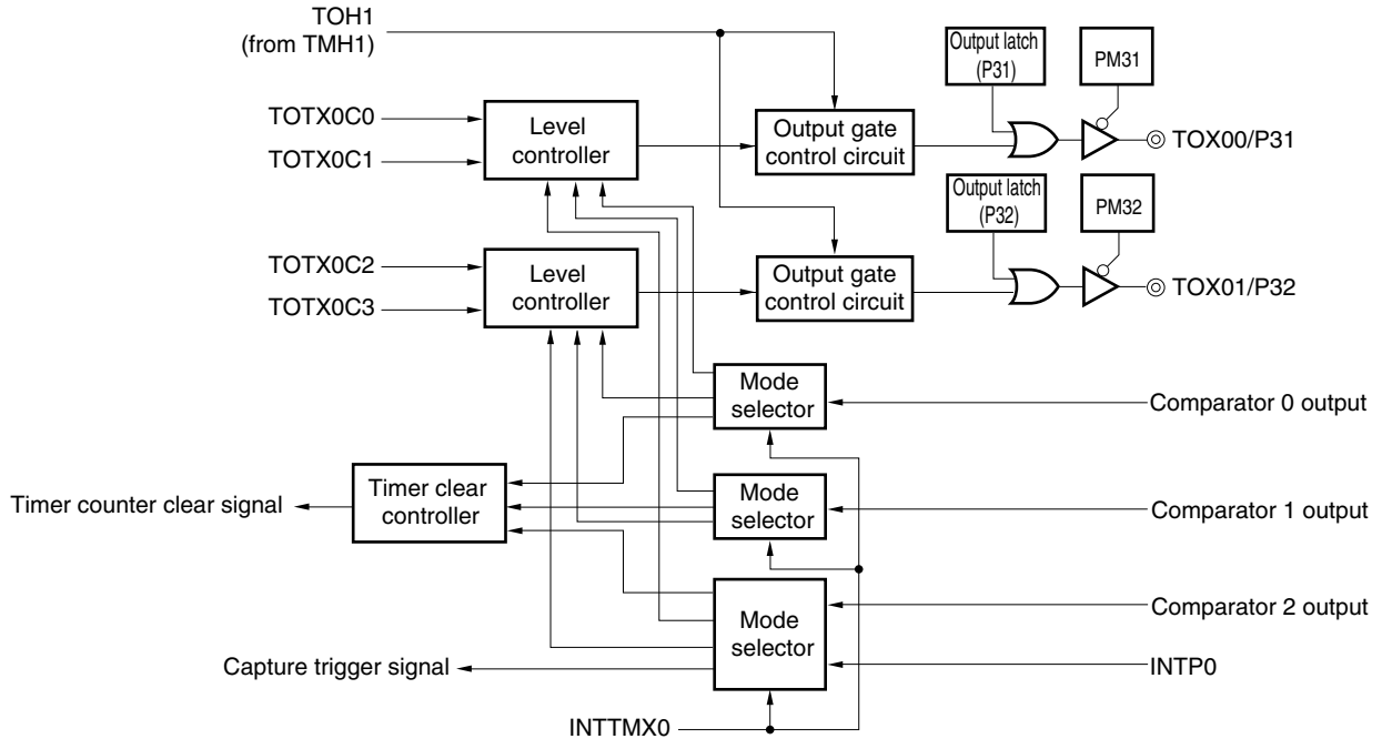
Figure 6-35. Block Diagram of 16-Bit Timer X1 Output Configuration
