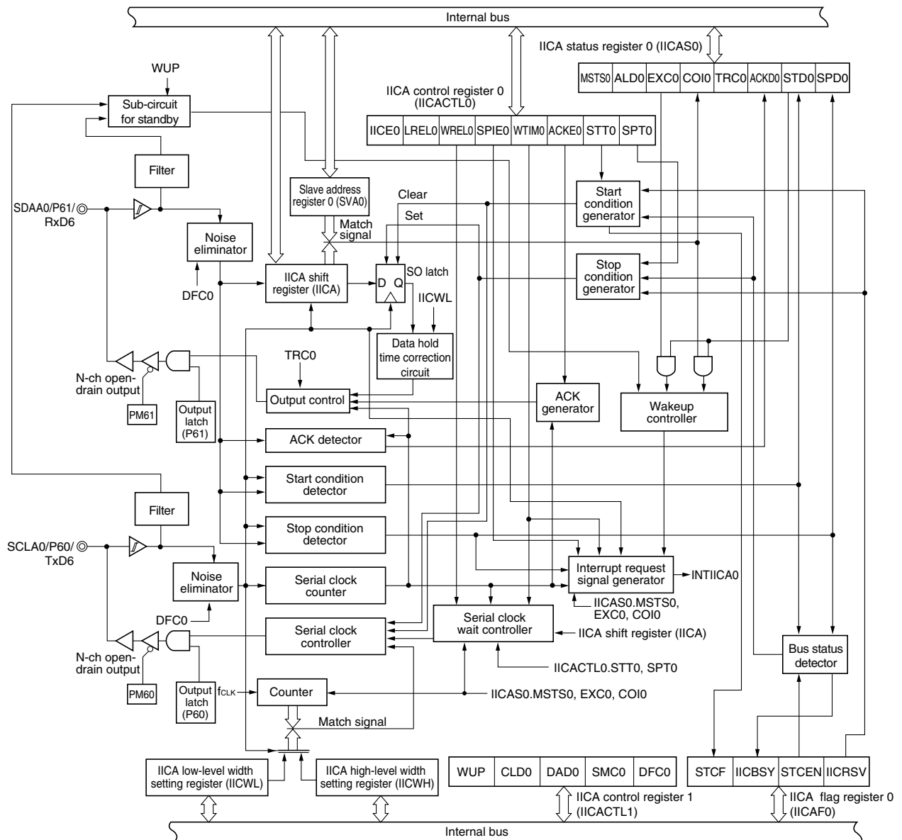
Figure 15-1. Block Diagram of Serial Interface IICA
