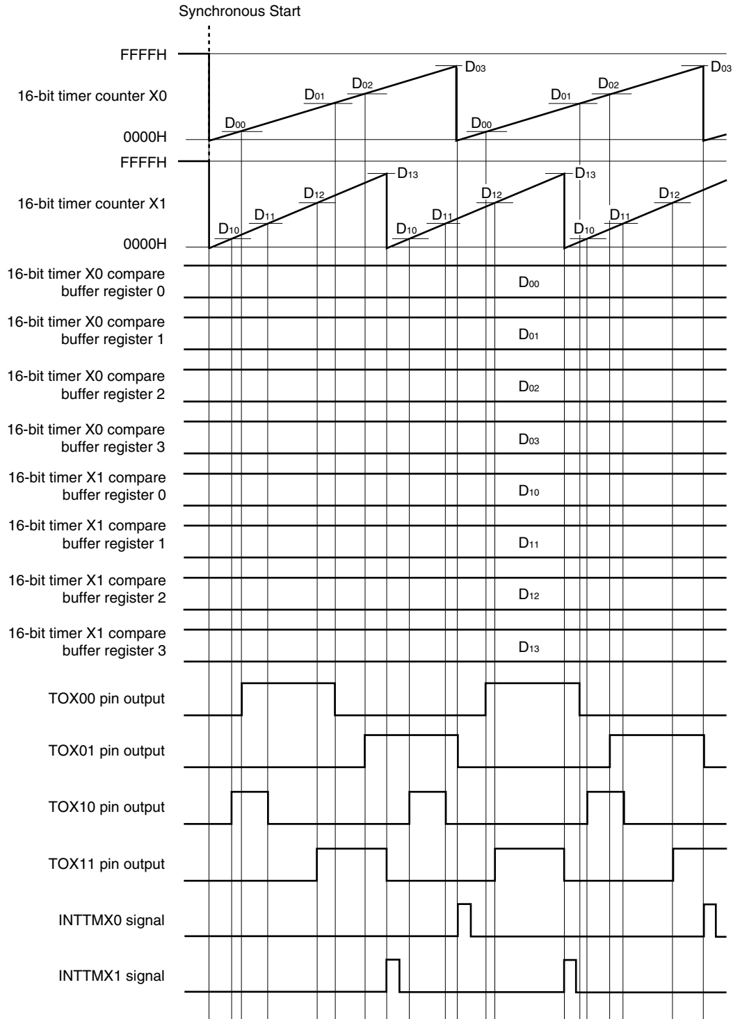
Figure 6-25. PWM Output Timing (TMX0 and TMX1 Synchronous Start mode, PWM Output: TOX00, TOX01, TOX10, and TOX11 Pins)
