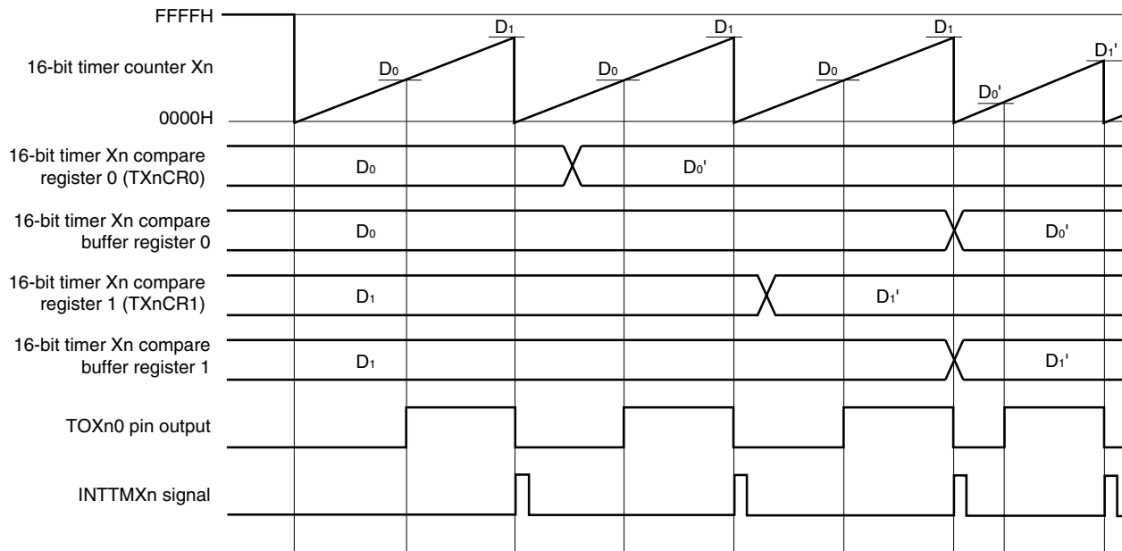
Figure 6-19. PWM Output Timing (TMXn-only Operation, PWM output: TOXn0 pin)
