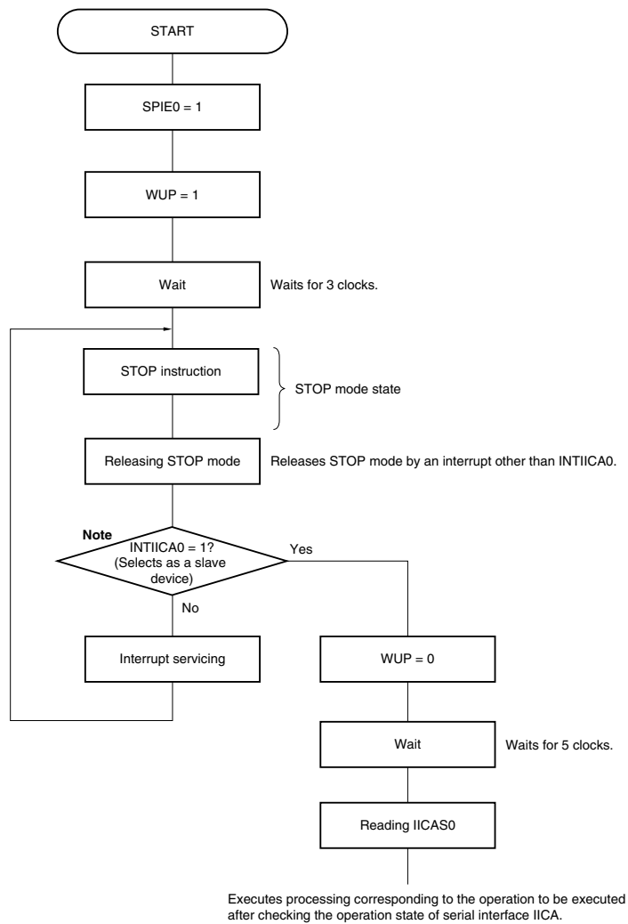
Figure 15-26. When Operating as Slave Device after Releasing STOP Mode other than by INTIICA0 (When Not Required to Operate as Master Device)
