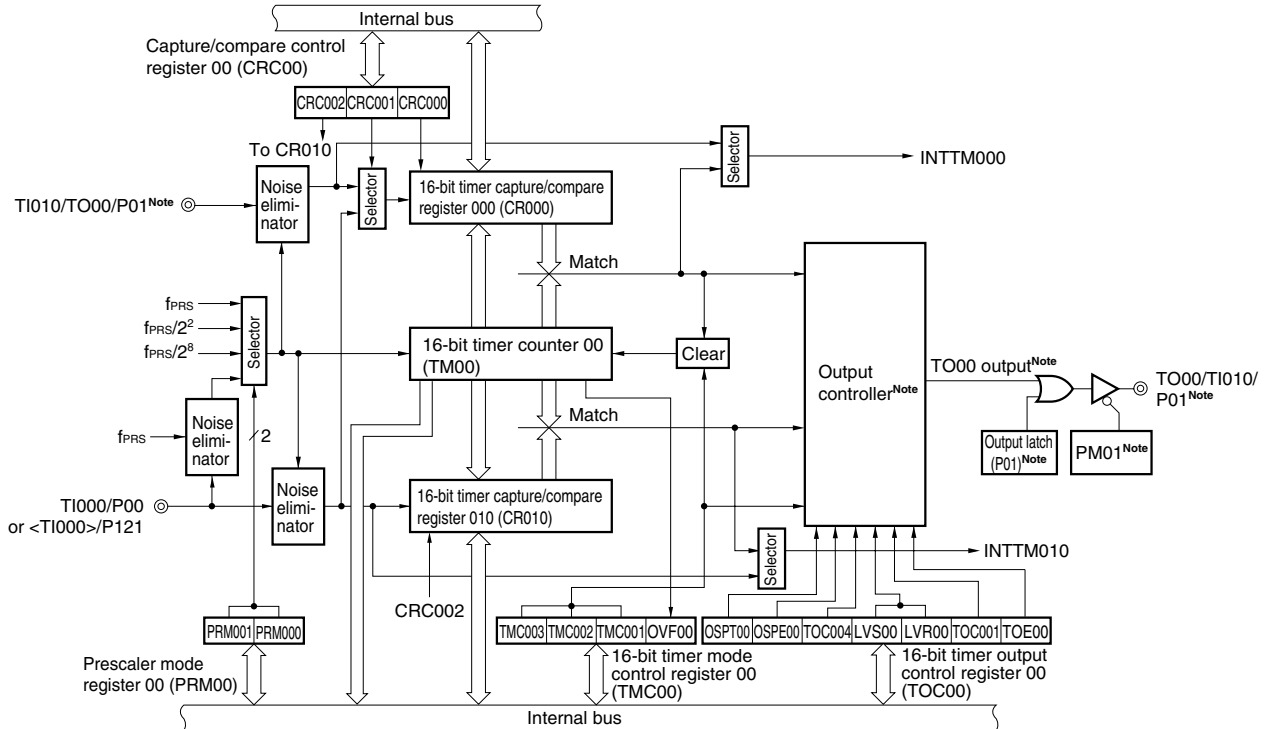
Figure 7-1. Block Diagram of 16-Bit Timer/Event Counter 00
