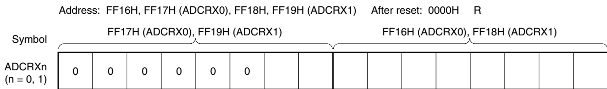
Figure 11-8. Format of 10-Bit A/D Conversion Result Register for TMXn Synchronization (ADCRXn)
