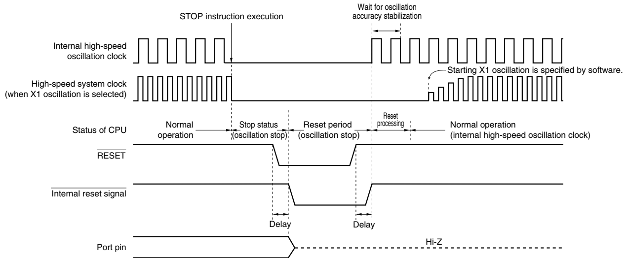
Figure 20-4. Timing of Reset in STOP Mode by RESET Input
