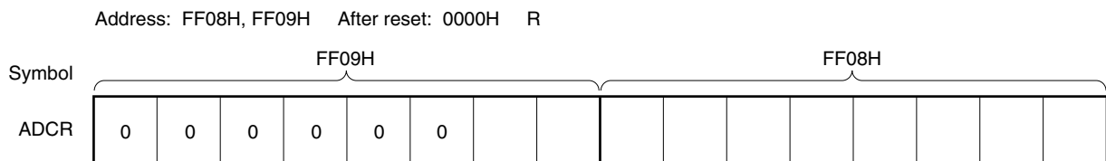
Figure 11-5. Format of 10-Bit A/D Conversion Result Register (ADCR)
