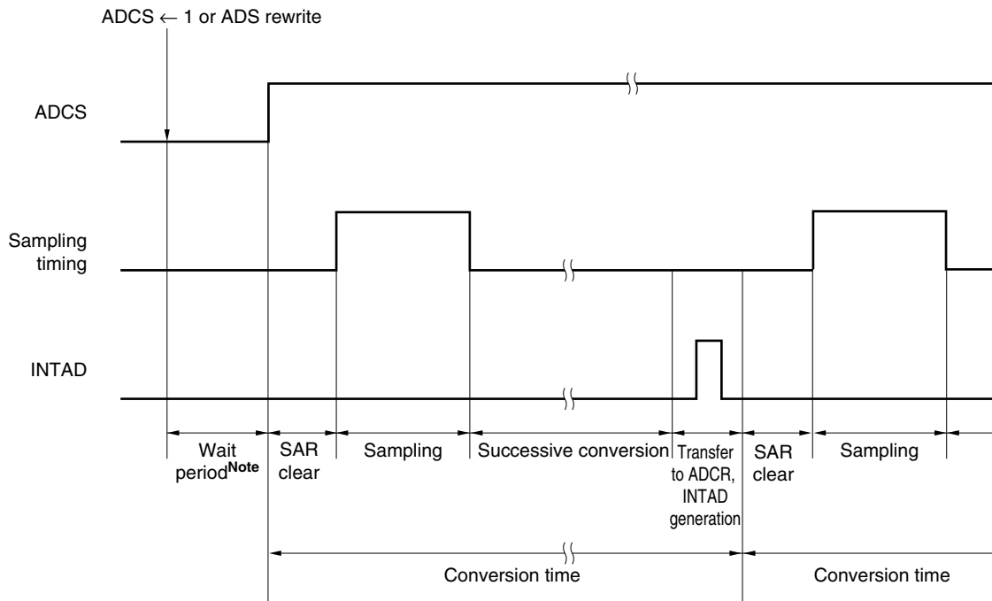
Figure 11-4. A/D Converter Sampling and A/D Conversion Timing
