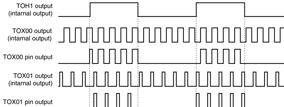
Figure 6-27. PWM Output Timing (TMX0-Only Operation (Dual Output), PWM Output from TOX00 and TOX01 When TOH1 Output Is at High Level)
