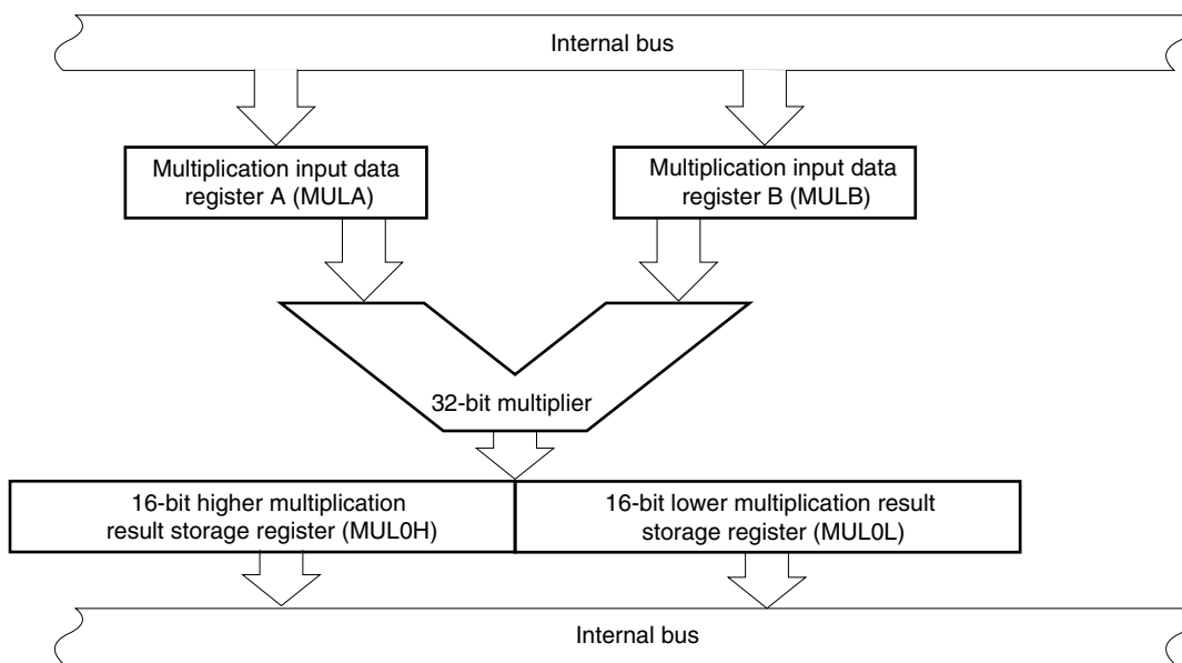
Figure 17-1. Block Diagram of Multiplier
