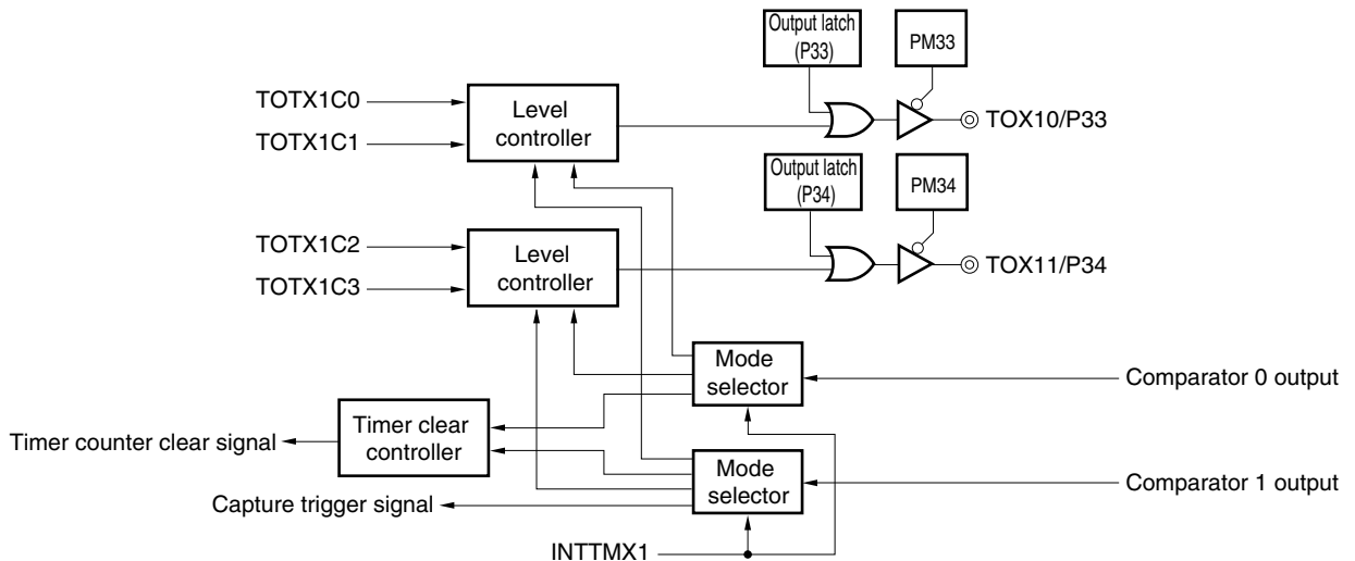
Figure 6-35. Block Diagram of 16-Bit Timer X1 Output Configuration
