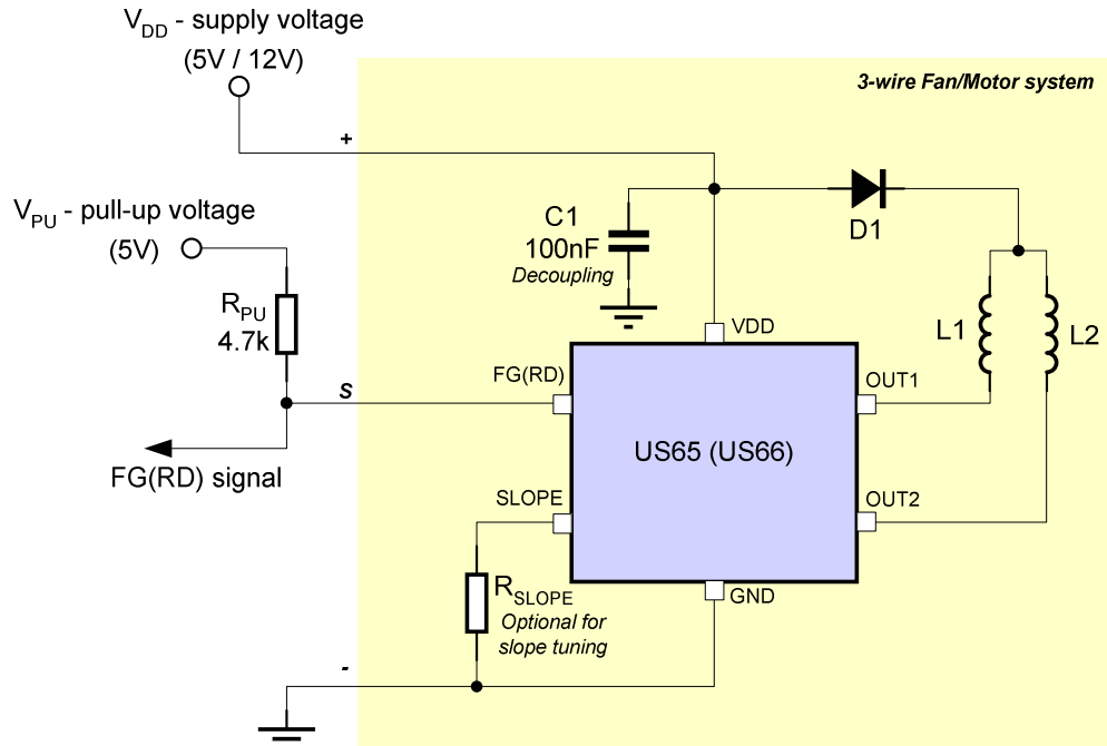
Typical computer fan application circuit
