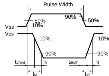
Fig.1-2 Switching Waveforms
