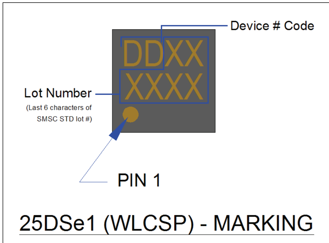
Figure 12.6 25-Ball WLCSP Package Marking
