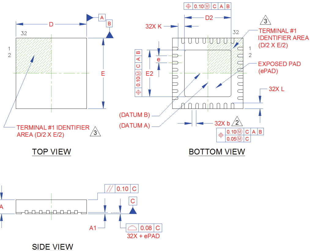
Figure 12.7 32-SQFN Package
