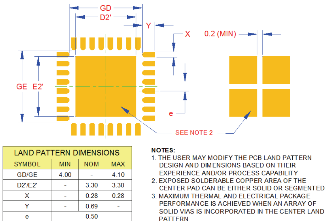
Figure 12.8 Recommended PCB Land Pattern
