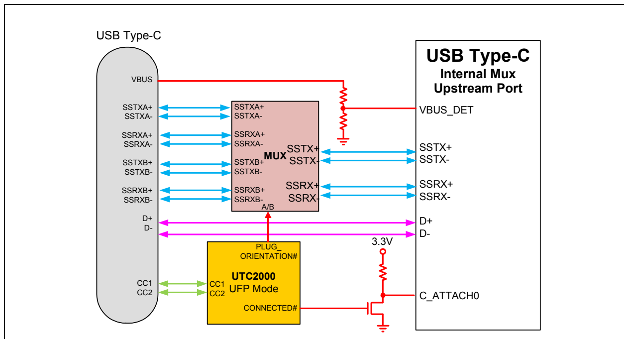
FIGURE 8-2: UFP TYPE-C PORT WITH MICROCHIP UTC2000 & INTERNAL MUX
