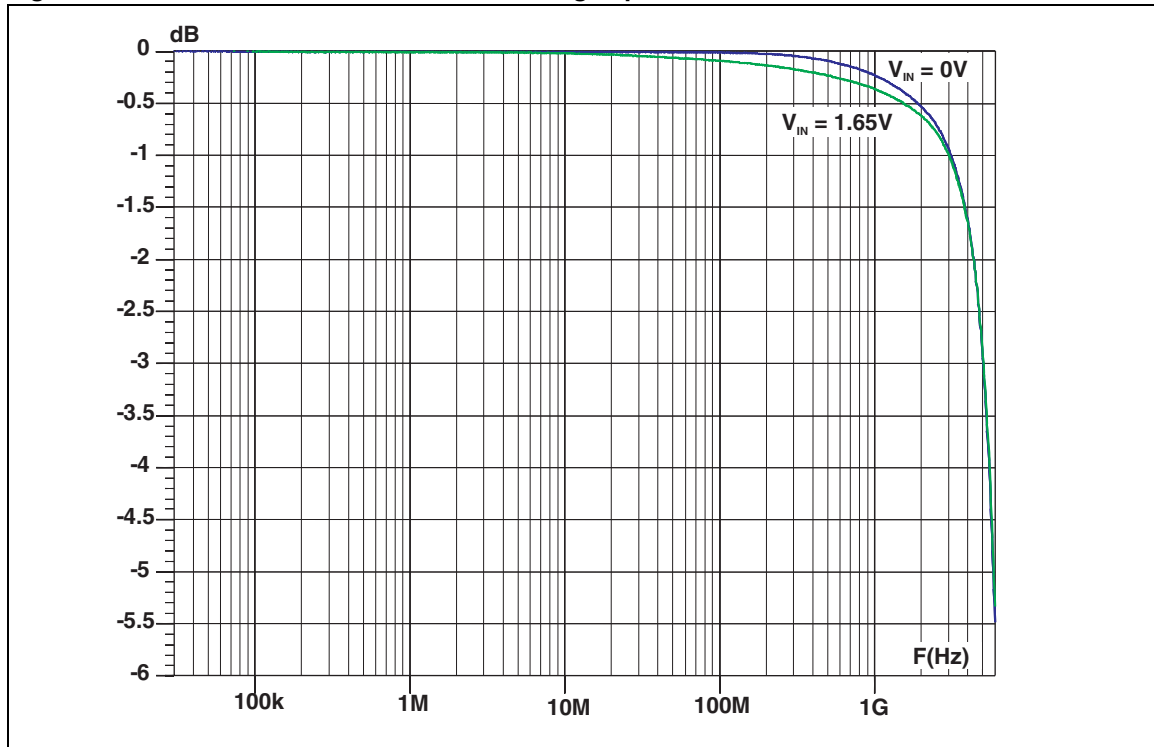
Figure 2. S21 attenuation measurement on high speed lines
