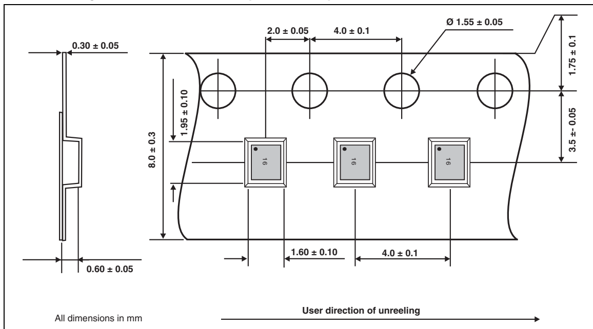
Figure 21. Micro QFN-8L tape and reel specifications
