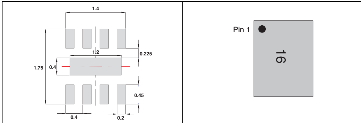
Figure 19. Foot print recommendations (dimensions in mm)
