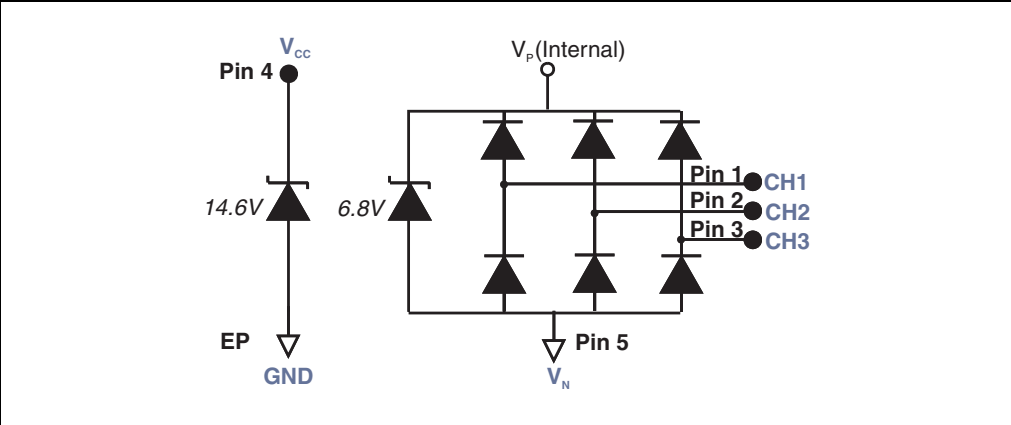
Figure 4. Typical application
