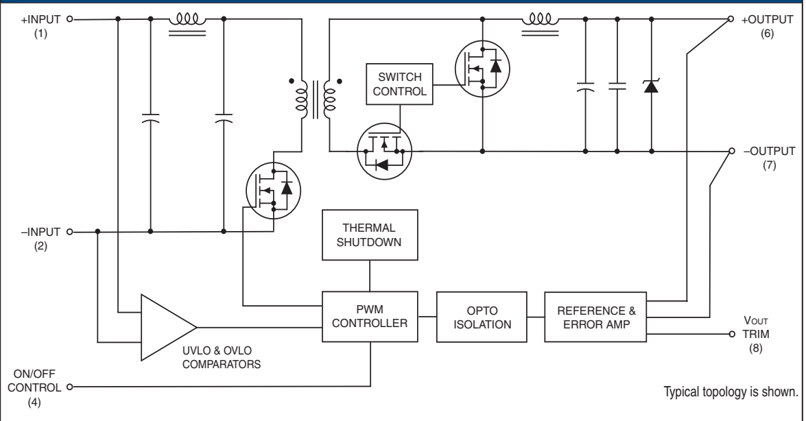
FIGURE 1. SIMPLIFIED SCHEMATIC
