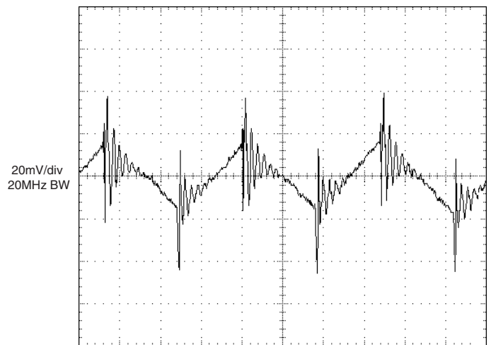
UWR-3.3/9-D48A Output Ripple and Noise (PARD)
