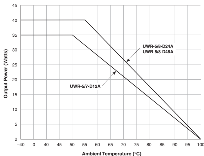
5V OUT Temperature Derating – Natural Convection
