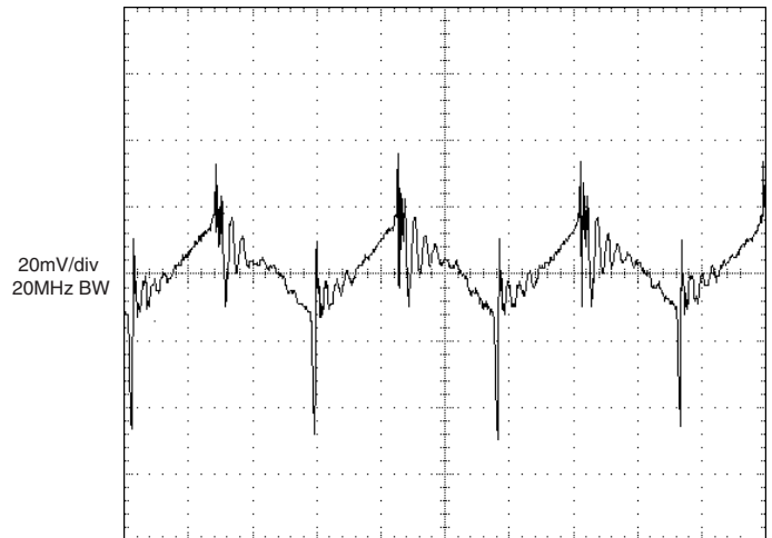
UWR-3.3/9-D24A Output Ripple and Noise (PARD)
