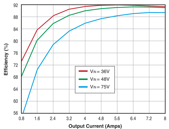
UWR-5/8-D48 Efficiency vs. Load @ 25°C Ambient
