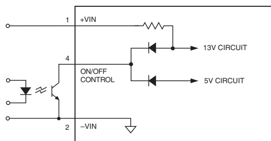
Figure 2. Driving the Positive Logic On/Off Control Pin
