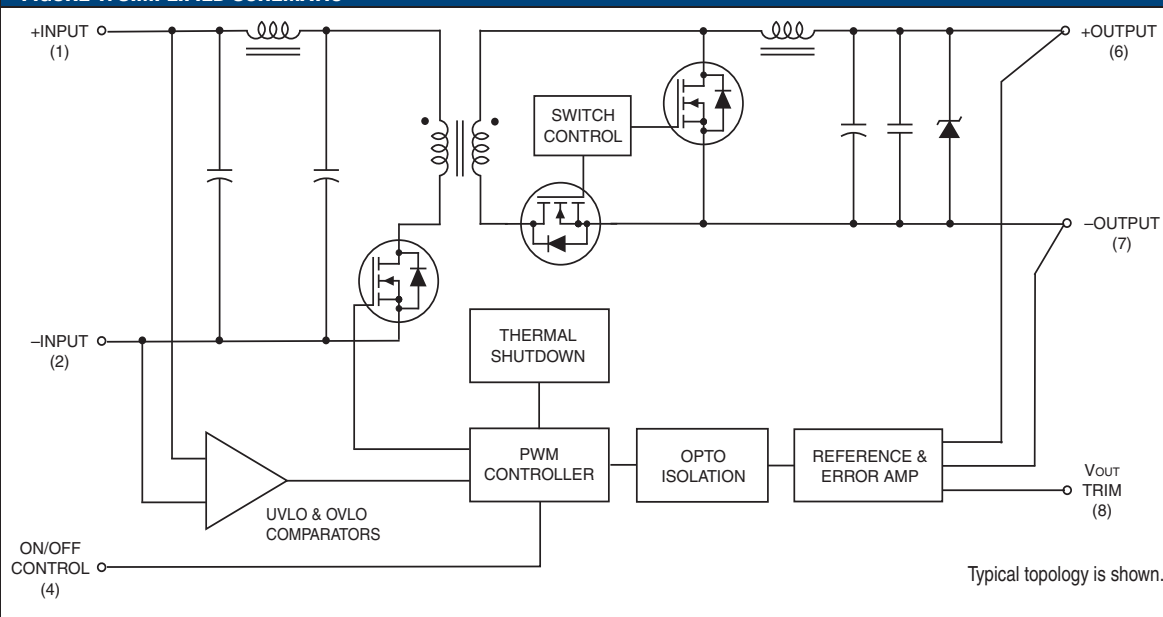
FIGURE 1. SIMPLIFIED SCHEMATIC
