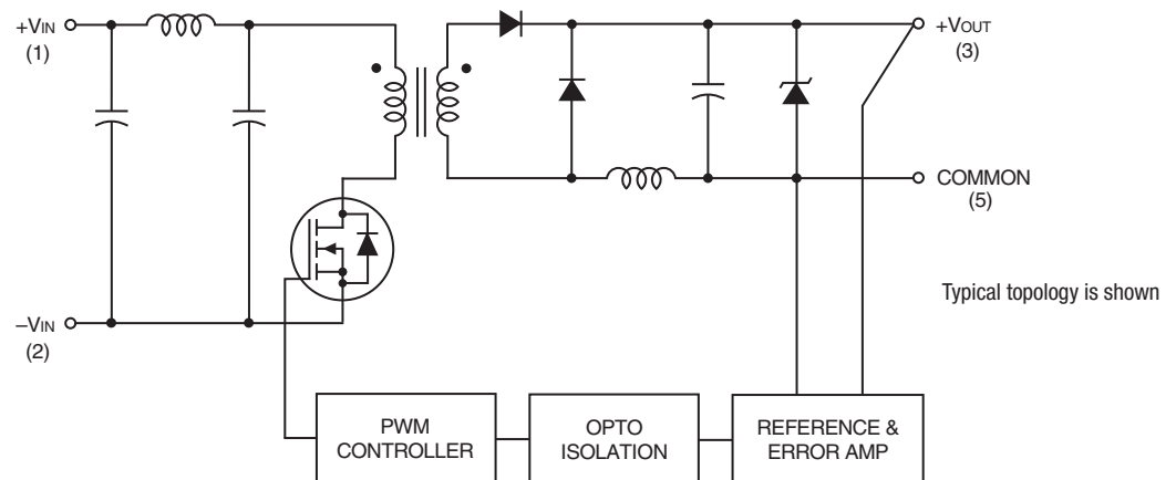
Figure 1. Simplified Schematic
