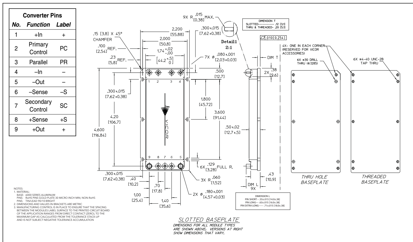
Figure 13 — Module outline
