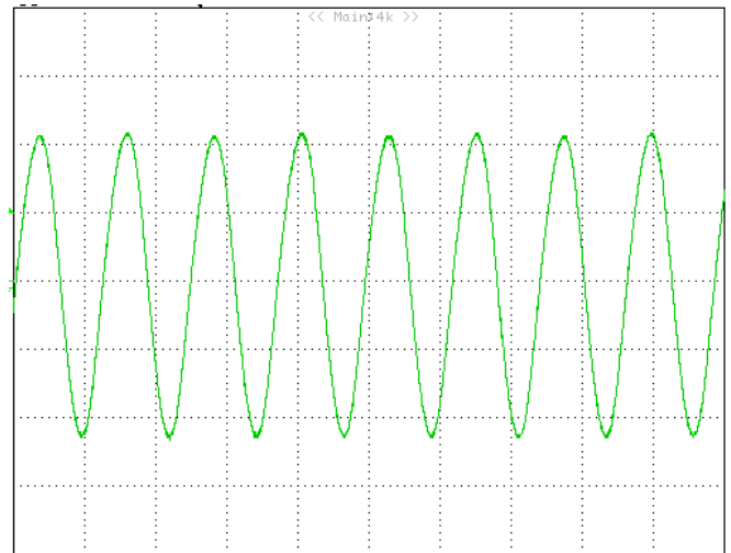
Figure 11: Input Terminal Ripple Current, i_c , at max output current and nominal input voltage with 12\mu H source impedance and 33\mu F electrolytic capacitor (100 mA/div, 2us/div).
