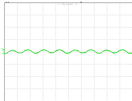
Figure 11: Input reflected ripple current, i_{si} , through a 12 \mu H source inductor at nominal input voltage and rated load current (20 mA/div, 2 \mu s/div)
