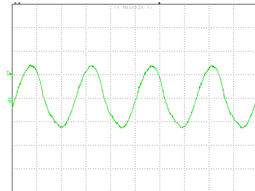
Figure 10: Input Terminal Ripple Current, i_c , at full rated output current and nominal input voltage with 12\mu\text{H} source impedance and 33\mu\text{F} electrolytic capacitor (200 mA/div, 1us/div)
