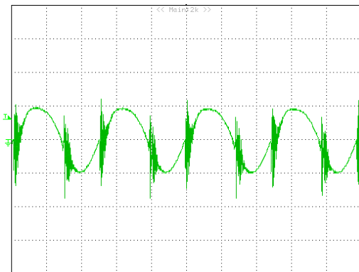
Figure 11: Input reflected ripple current, i_{si} , through a 12 \mu H source inductor at nominal input voltage and rated load current (20 mA/div, 2 \mu s/div)
