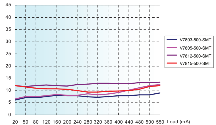
Output Voltage Ripple VS Output Load ( V_{in} =Norm)
