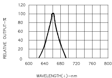
Fig.1 SPECTRAL RESPONSE
