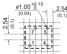
PIN CONNECTIONS
