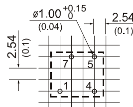
PIN CONNECTIONS
