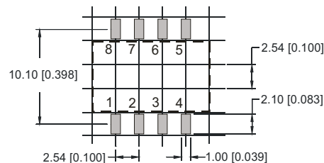
RECOMMENDED FOOTPRINT Top view, grid: 2.54mm(0.1inch)
