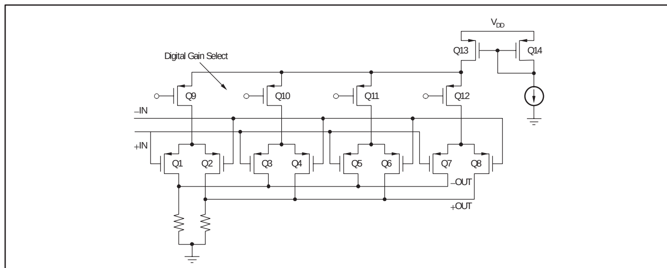
Figure 55. Programmable LNP
