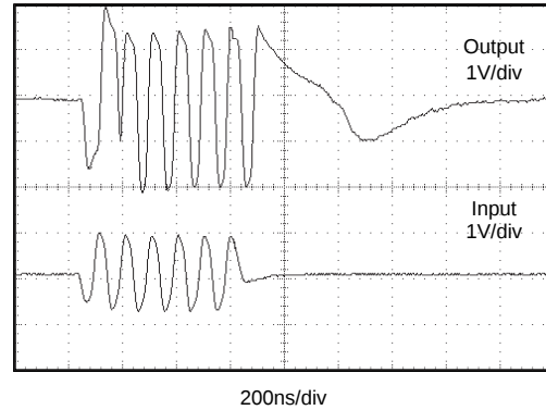
OVERLOAD RECOVERY (Differential, V_{CA\_CNTRL} = 3.0\text{V} , \text{MGS} = 111 )
