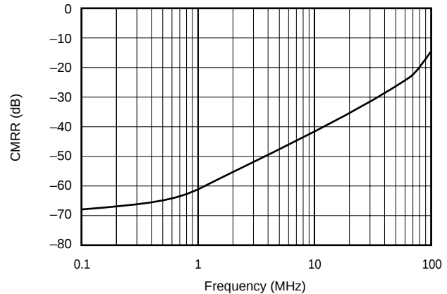
CMRR vs FREQUENCY (LNP only)
