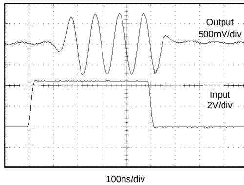
GAIN RESPONSE (Differential, V_{CA\_CNTRL} Pulsed, \text{MGS} = 111 )
