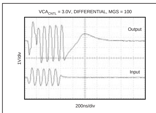
FIGURE 13. Overload Recovery Response For Maximum Gain.
