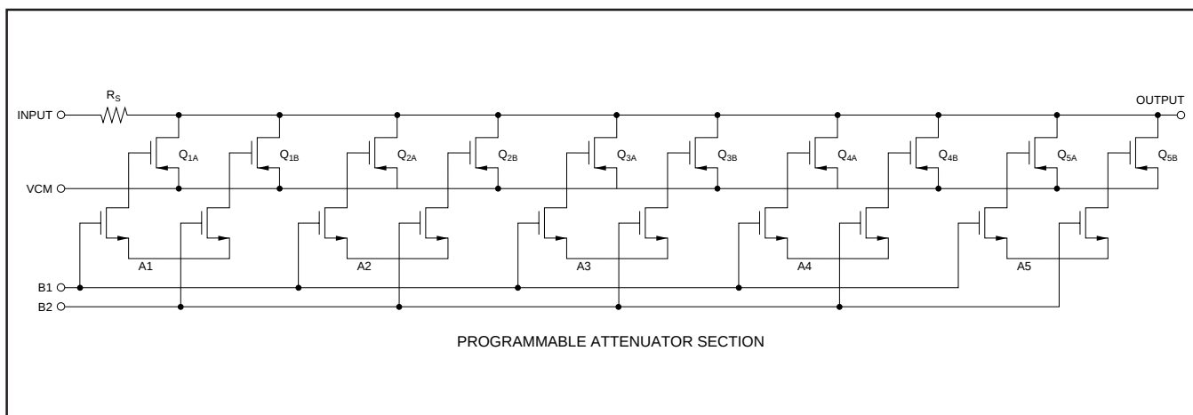
FIGURE 10. Programmable Attenuator Section.
