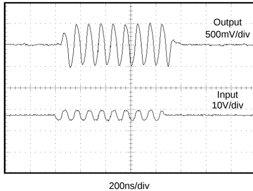
PULSE RESPONSE (BURSTS) (Differential, V_{CA\_CNTRL} = 3.0\text{V} , \text{MGS} = 111 )
