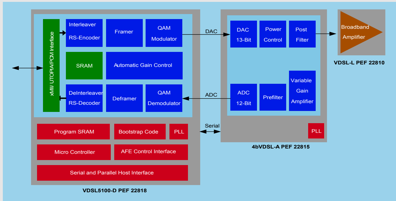
VDSL5100 Block Diagram
