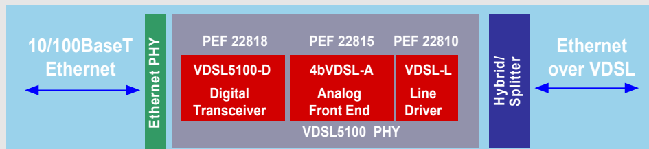
Ethernet over VDSL Linecard Application Example
