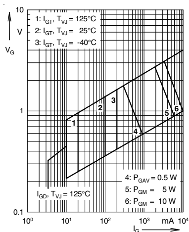
Fig. 3 Gate trigger characteristic
