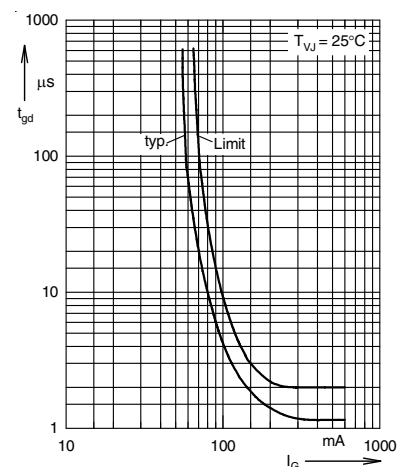
Fig. 1 Gate trigger delay time
