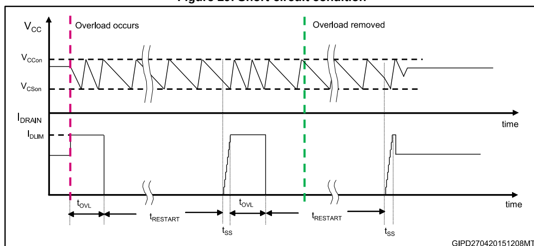
Figure 29: Short-circuit condition
