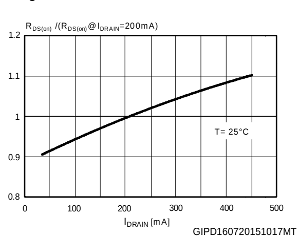
Figure 19: Static drain source on resistance
