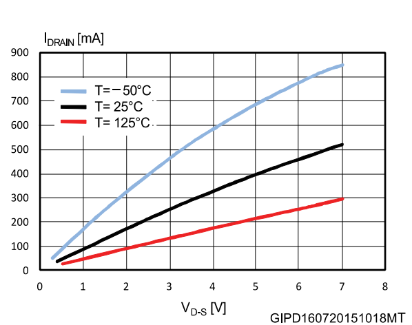
Figure 20: Output characteristic
