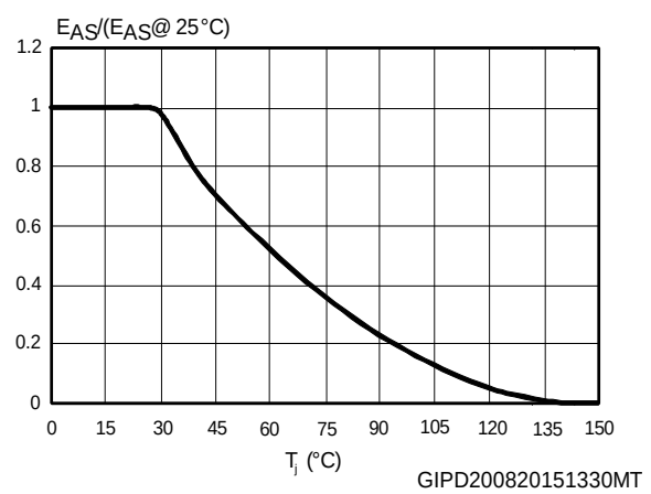
Figure 22: Max avalanche energy vs T_J
