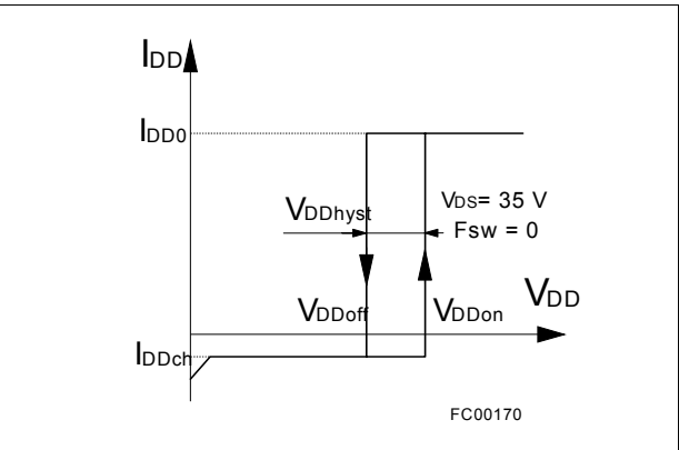
Figure 6. Undervoltage lockout
