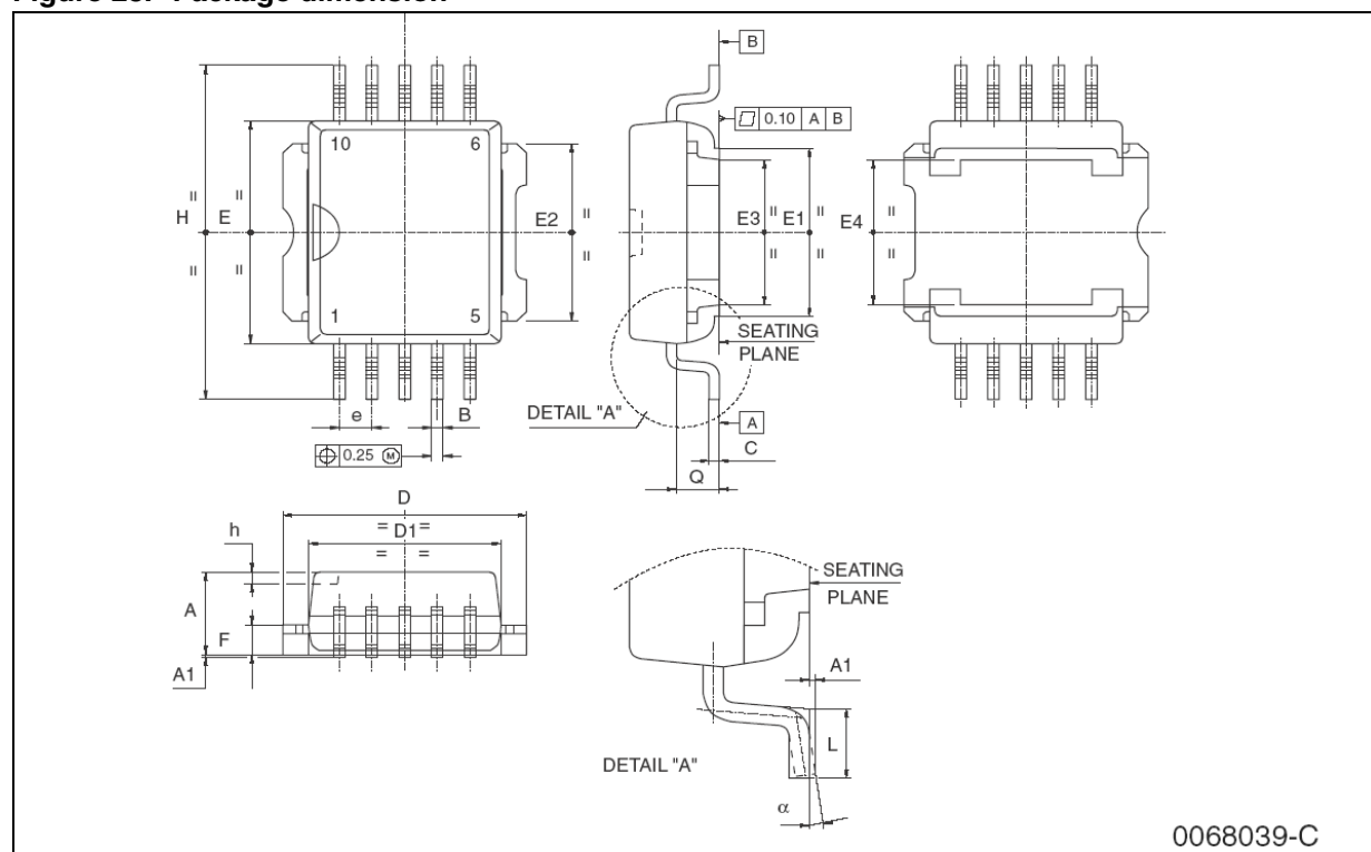
Figure 28. Package dimension
