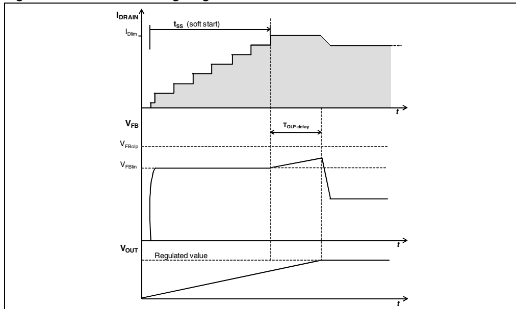
Figure 20. Soft-start: timing diagram
