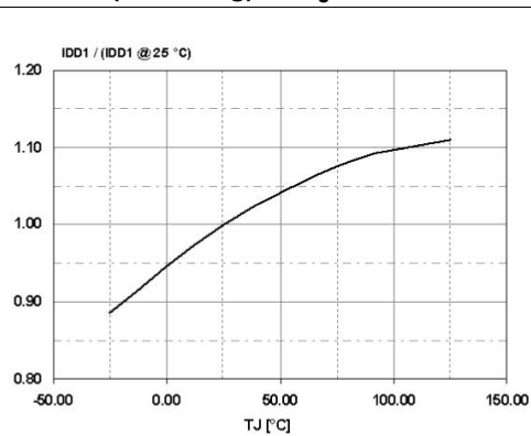
Figure 11. Operating supply current (switching) vs T_J
