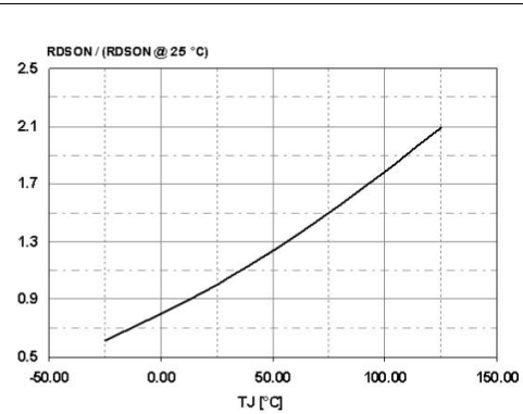
Figure 13. Power MOSFET on-resistance vs T_J
