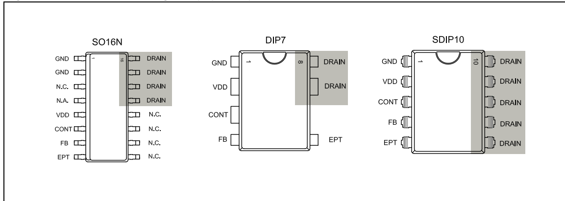
Figure 3. Connection diagram (top view)
