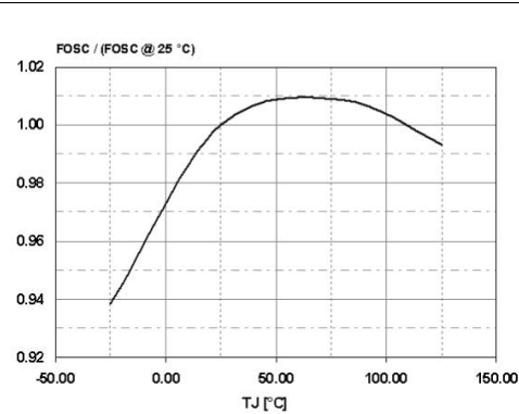
Figure 7. Switching frequency vs T_J
