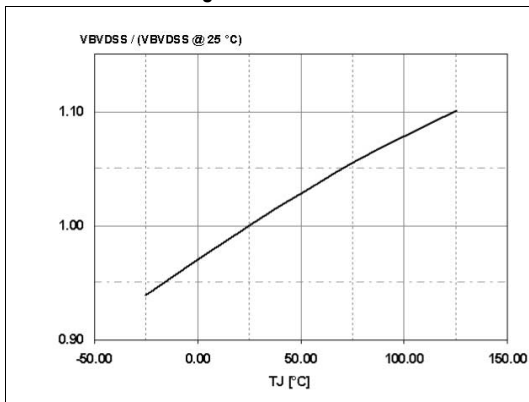
Figure 14. Power MOSFET break down voltage vs T_J
