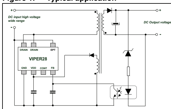
Figure 1. Typical application
