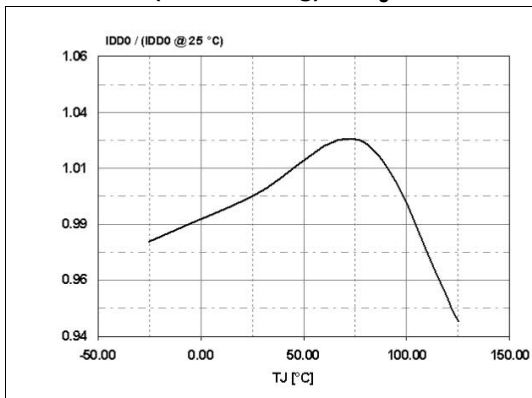
Figure 10. Operating supply current (no switching) vs T_J
