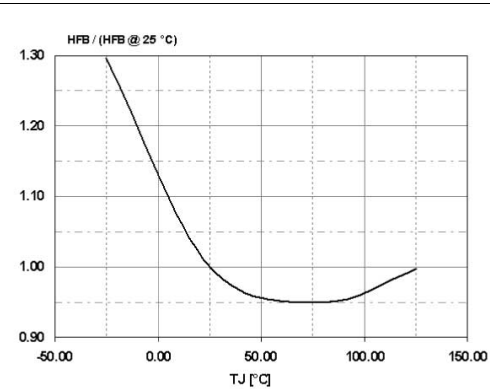
Figure 9. HFB vs T_J
