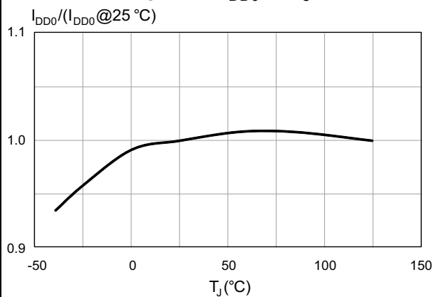
Figure 12. I_{DD0} vs T_J
