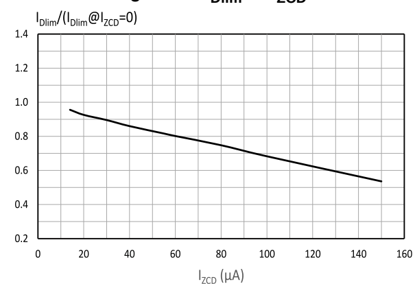
Figure 15. I_{Dlim} vs I_{ZCD}
