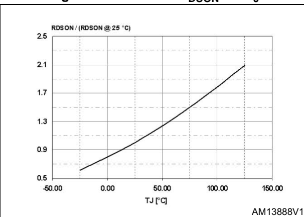
Figure 11. Main FET R_{DS(on)} vs. T_J
