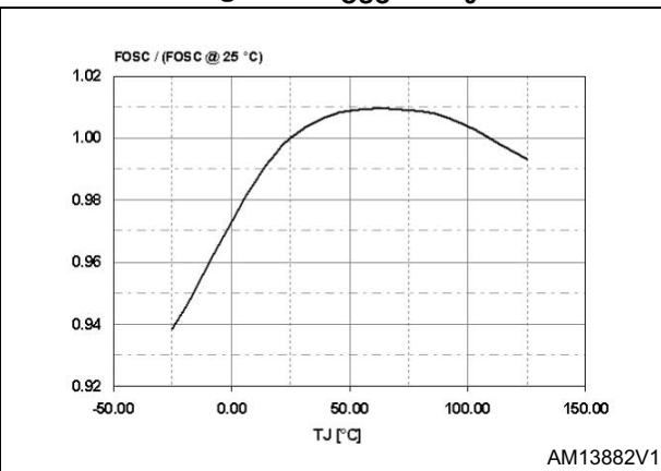
Figure 7. F_{OSC} vs. T_J
