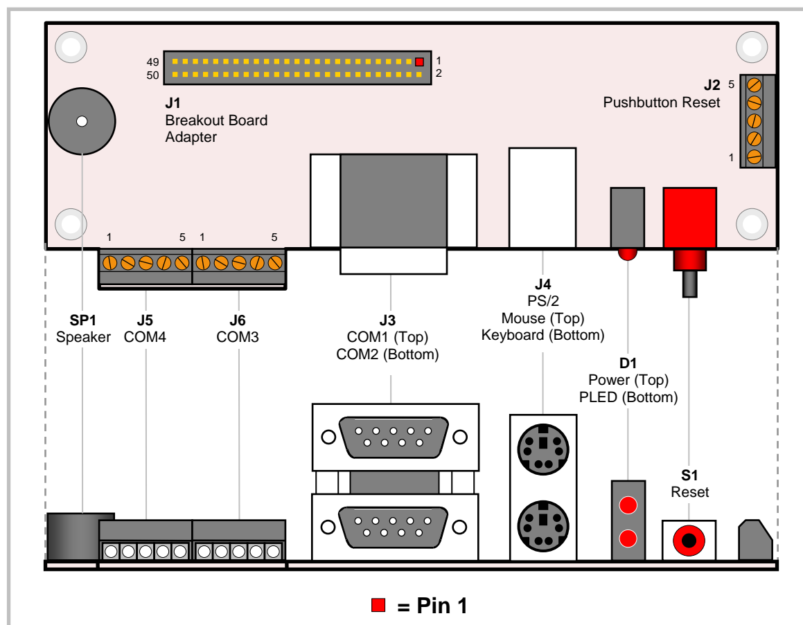
Figure 9. VL-CBR-5009 Connectors
