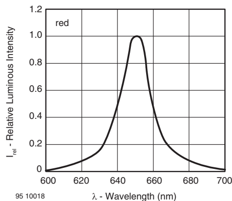
Fig. 4 - Relative Luminous Intensity vs. Wavelength
