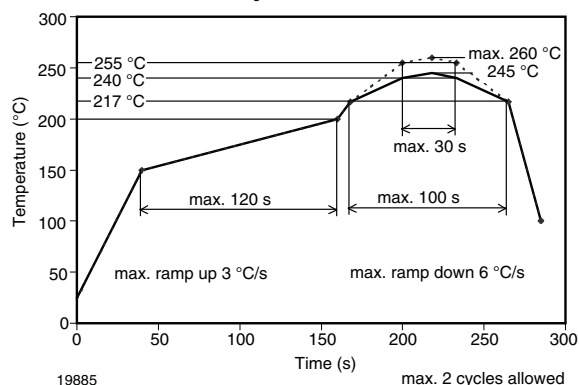
Fig. 13 - Vishay Lead (Pb)-free Reflow Soldering Profile (acc. to J-STD-020C)
