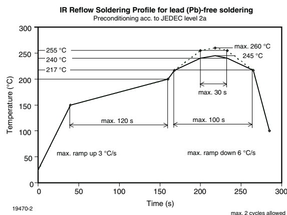
Fig. 12 - Vishay Leadfree Reflow Soldering Profile (acc. to J-STD-020)
