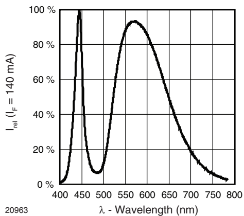
Fig. 9 - Relative Spectral Emission for Natural White
