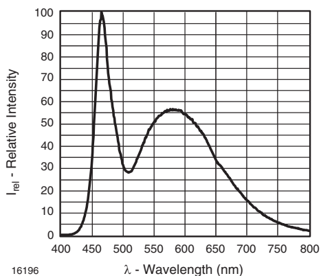
Fig. 8 - Relative Spectral Emission for Cool White
