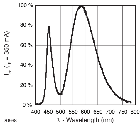
Fig. 10 - Relative Spectral Emission for Warm White
