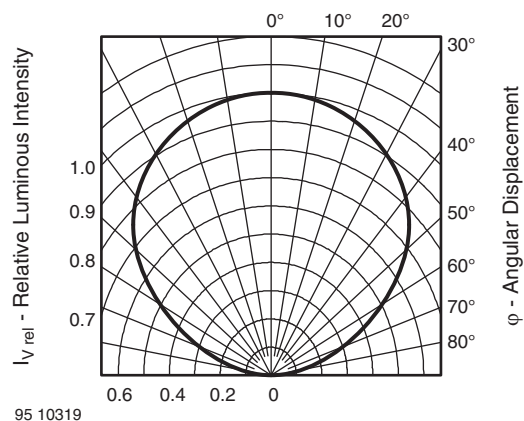
Fig. 11 - Relative Luminous Intensity vs. Angular Displacement
