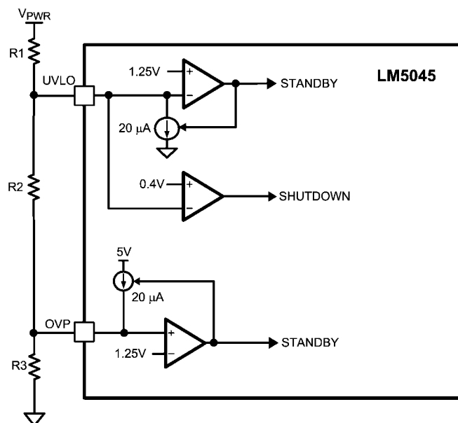
FIGURE 15. UVLO/OVP Divider
