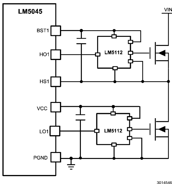
FIGURE 23. Using a Low Side Gate Driver to Augment Gate Drive Strength
