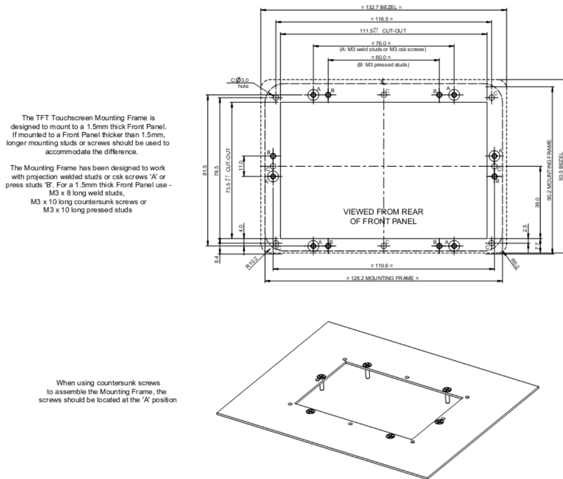
Figure 5-3 VM801P43A panel mount dimensions
