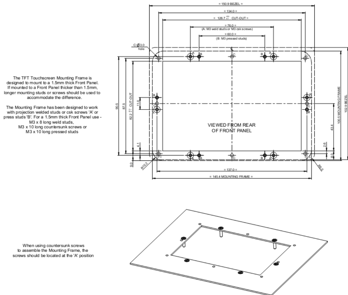
Figure 5-4 VM801P50A panel mount dimensions
