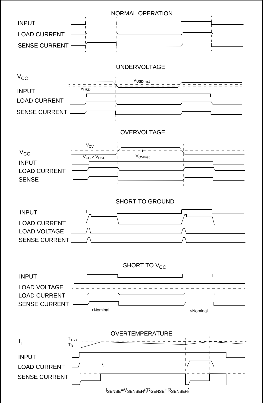
Figure 6. Waveforms
