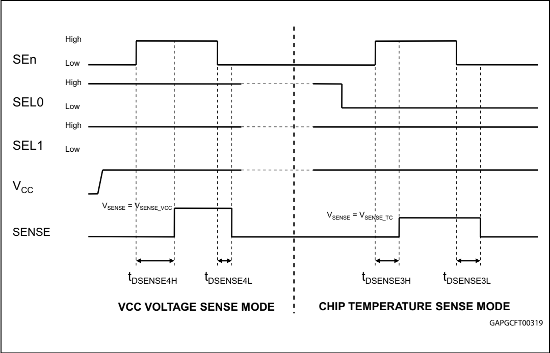
Figure 8. Multisense timings (chip temperature and V_{CC} sense mode)
