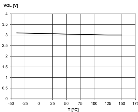
Figure 32. OFF-state open-load voltage detection threshold
