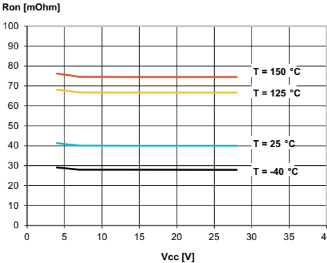
Figure 26. On-state resistance vs. V_{CC}
