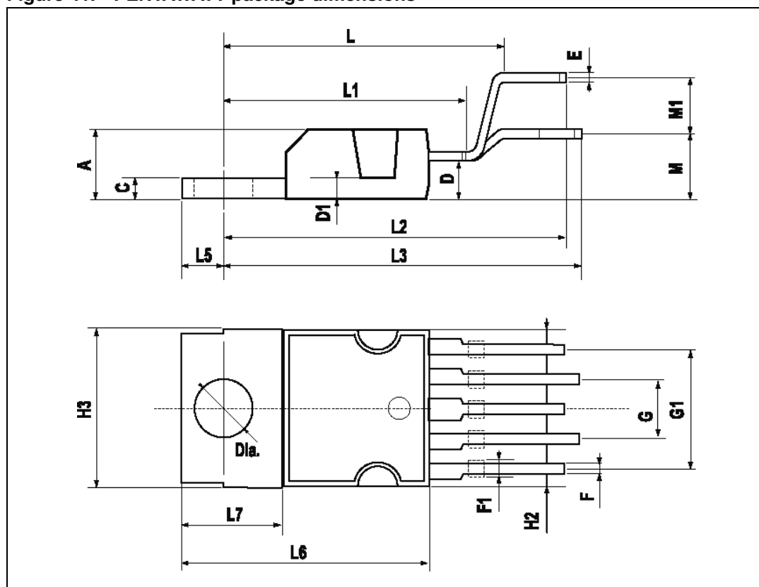
Figure 41. PENTAWATT package dimensions
